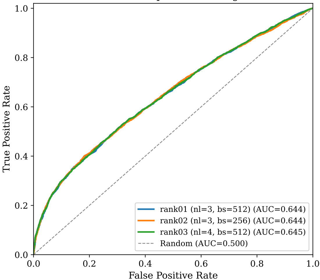
ROC Curves — Top-3 GNN Configurations
