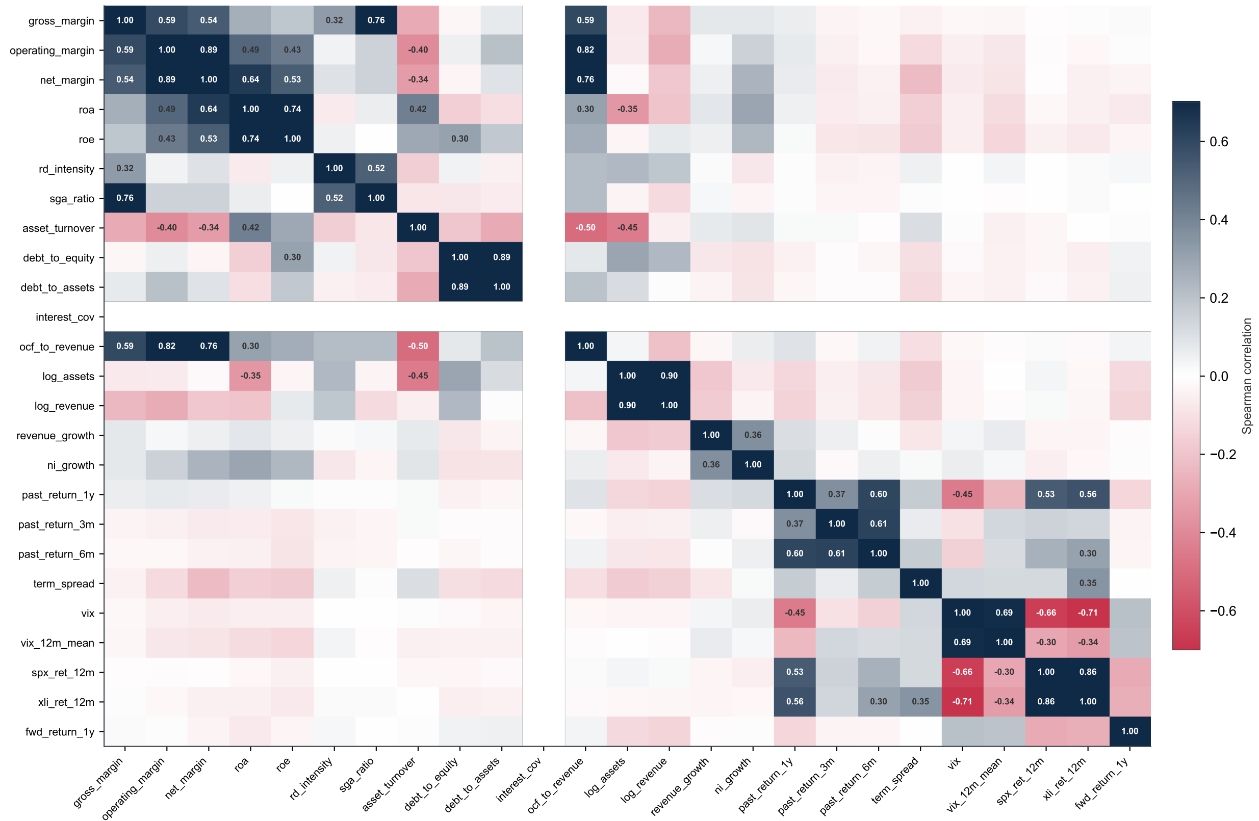
Feature correlation matrix (Spearman) | Industrials panel
