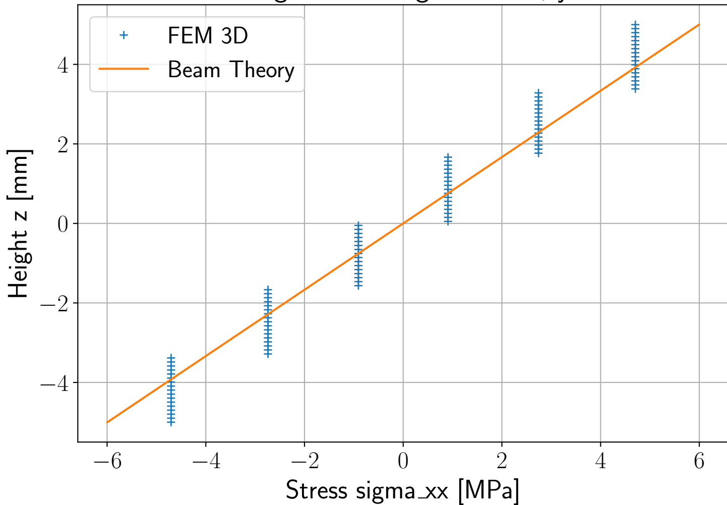
Stress \sigma_{xx} along z at x=1 , y=5.0
