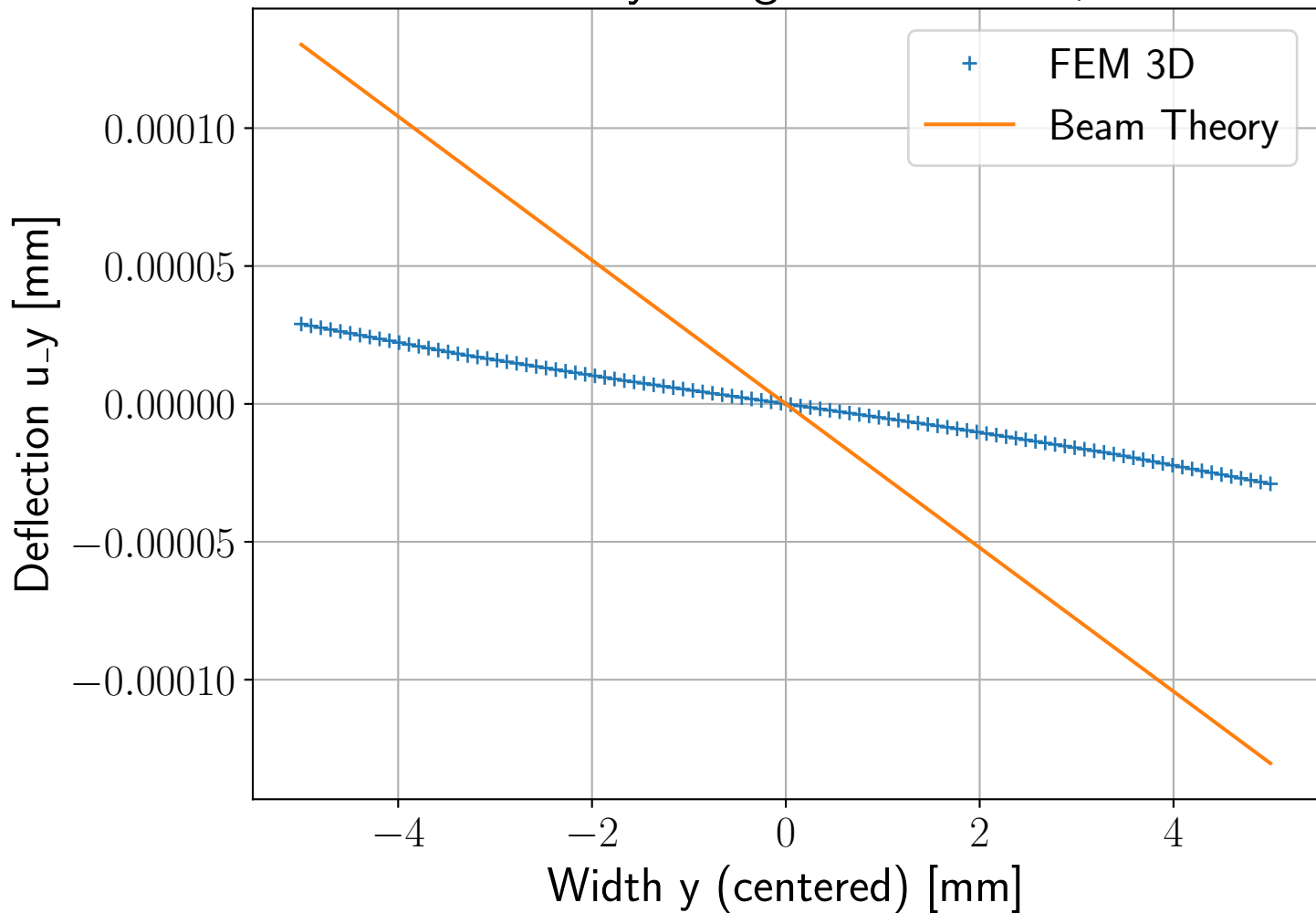
Deflection u_y along width at x=1 , z=10
