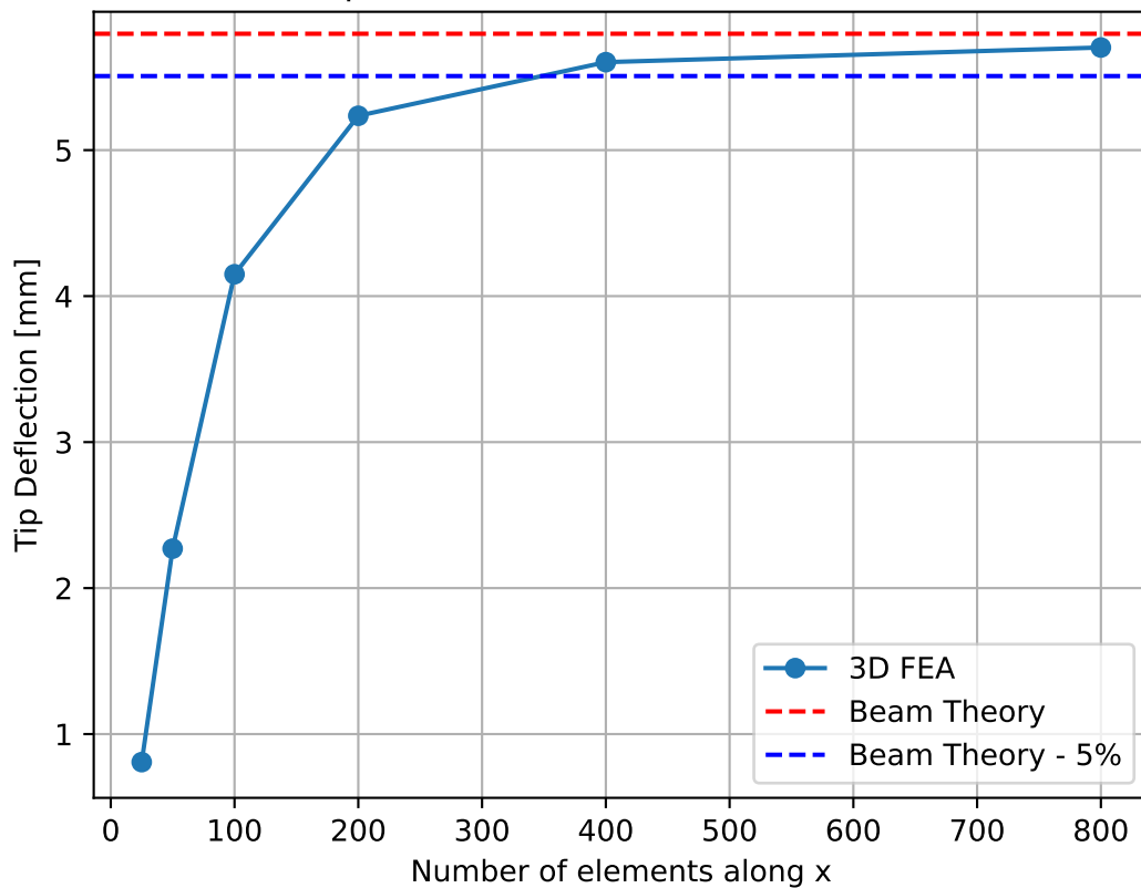
Tip Deflection vs Mesh Refinement
