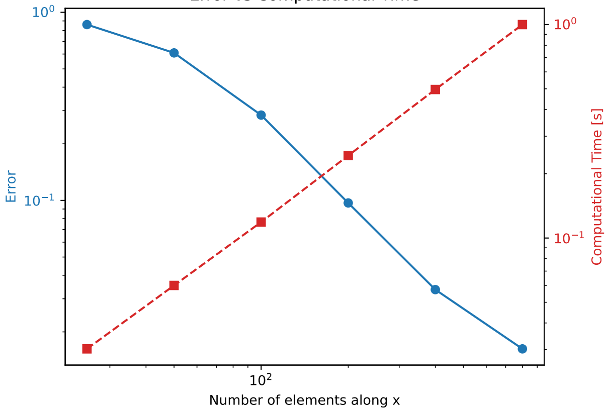
Error vs Computational Time
