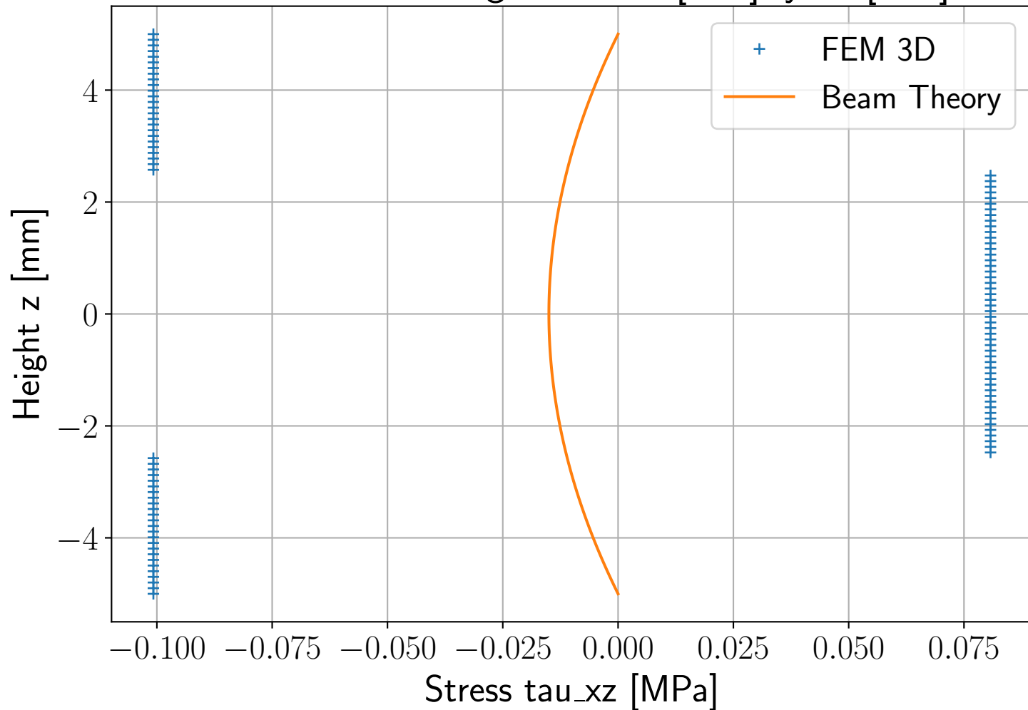
Stress \tau_{xz} along z at x=1 [mm], y=0 [mm]
