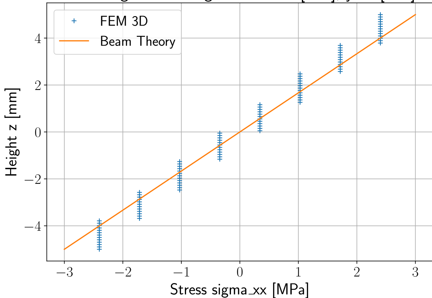
Stress \sigma_{xx} along z at x=500 [mm], y=0 [mm]
