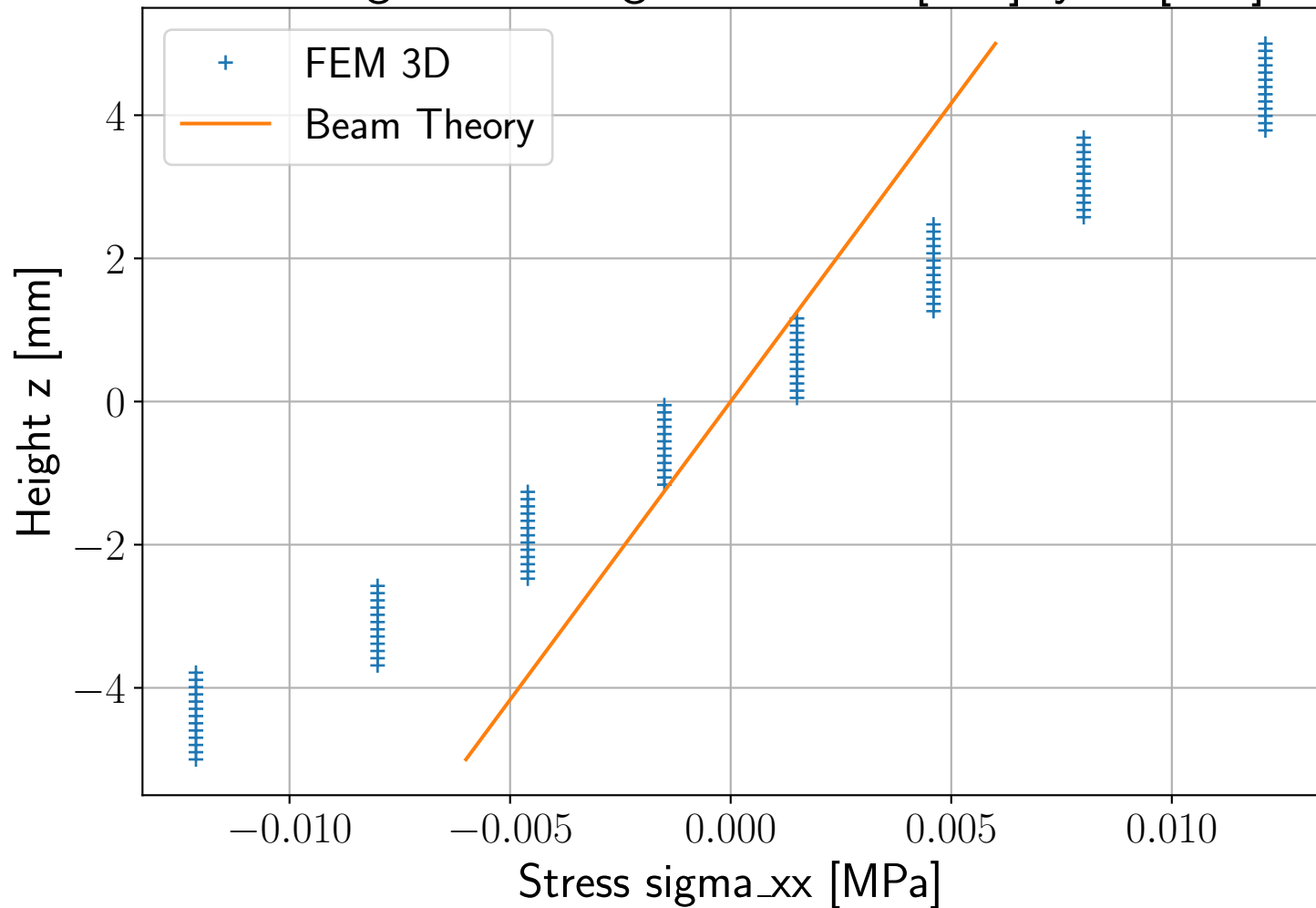
Stress \sigma_{xx} along z at x=999 [mm], y=0 [mm]
