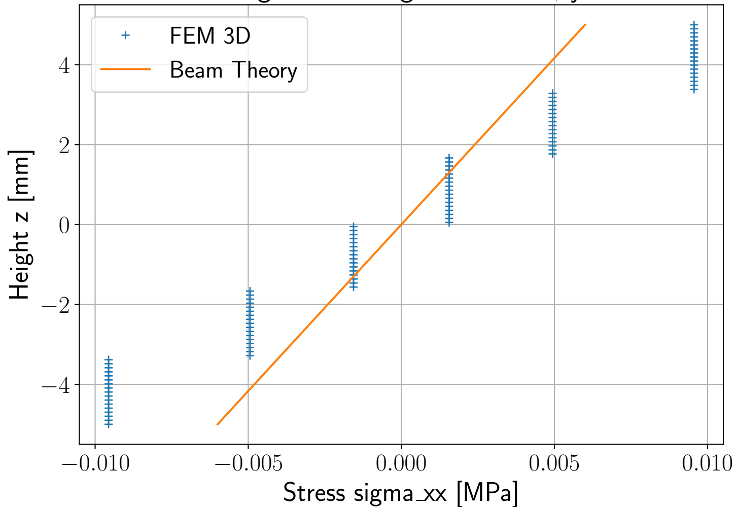
Stress \sigma_{xx} along z at x=999 , y=5.0
