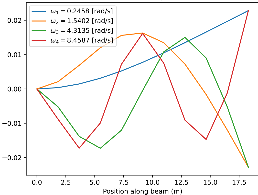
Mode 4 Shape
