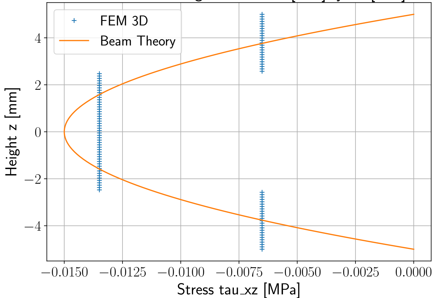
Stress \tau_{xz} along z at x=500 [mm], y=0 [mm]
