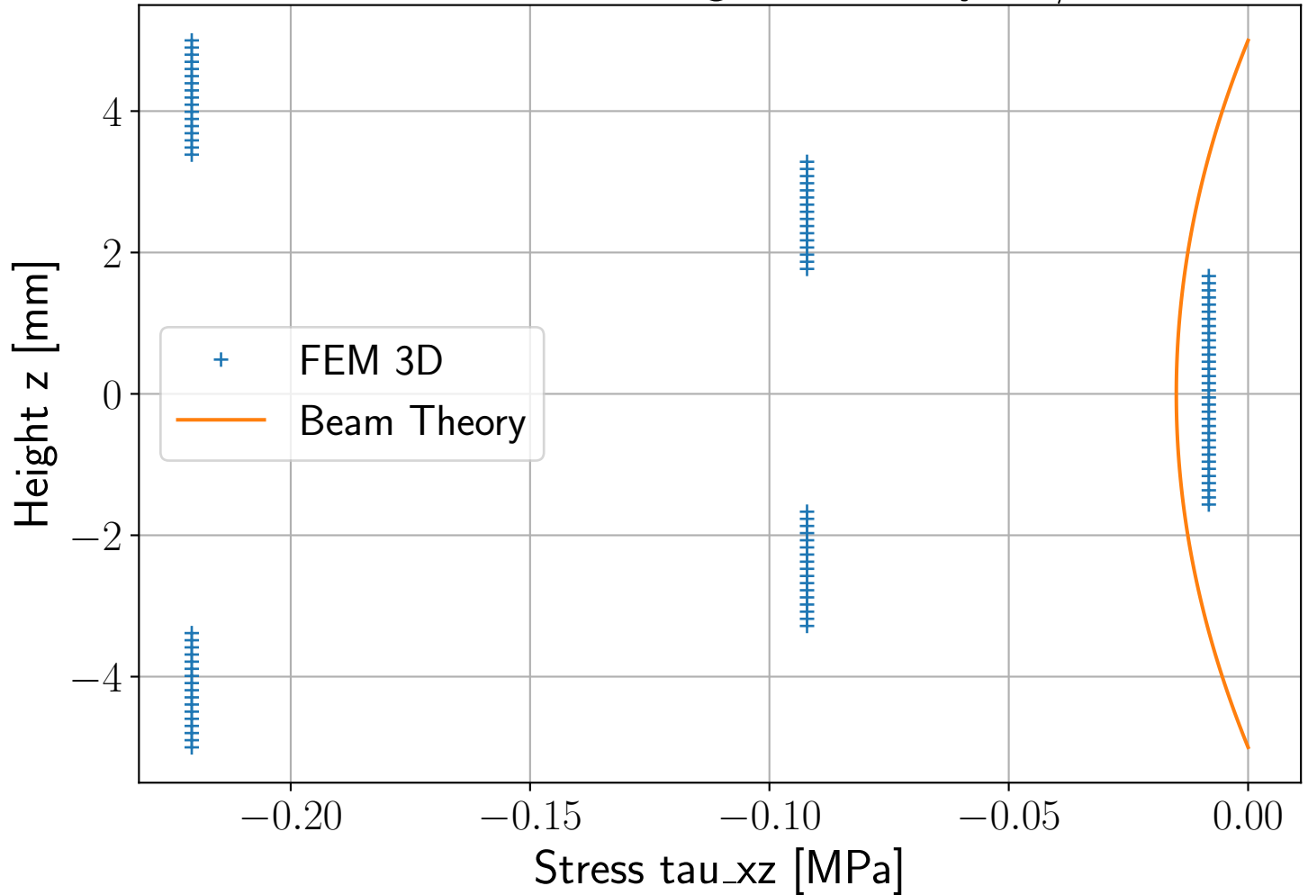
Stress \tau_{xz} along z at x=L , y=H/2
