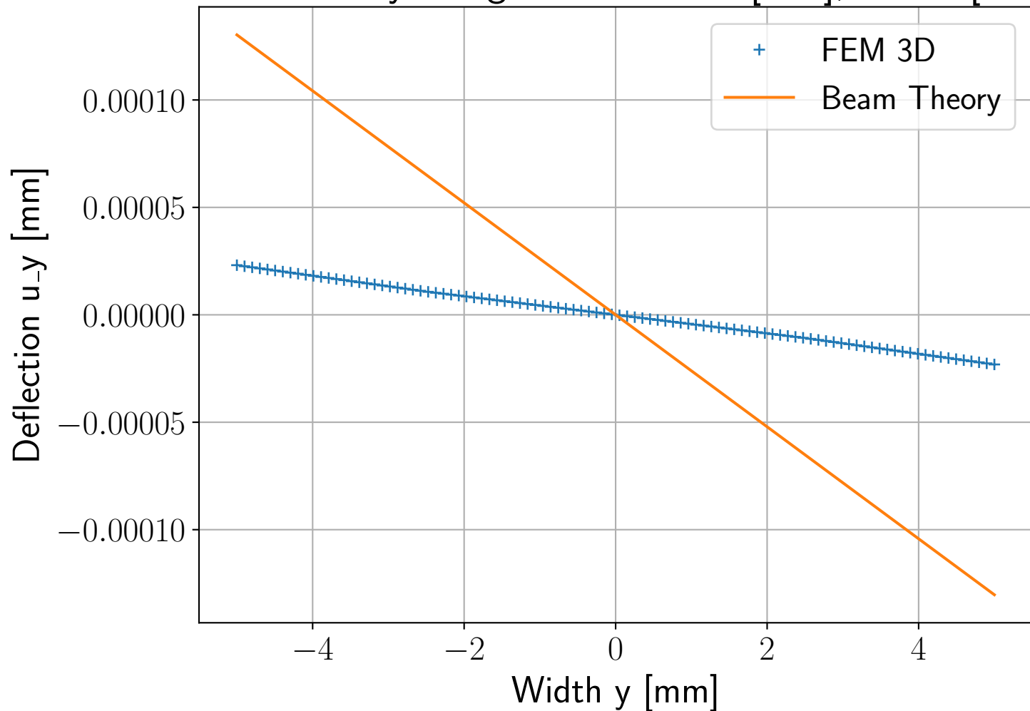
Deflection u_y along width at x=1 [mm], z=5.0 [mm]
