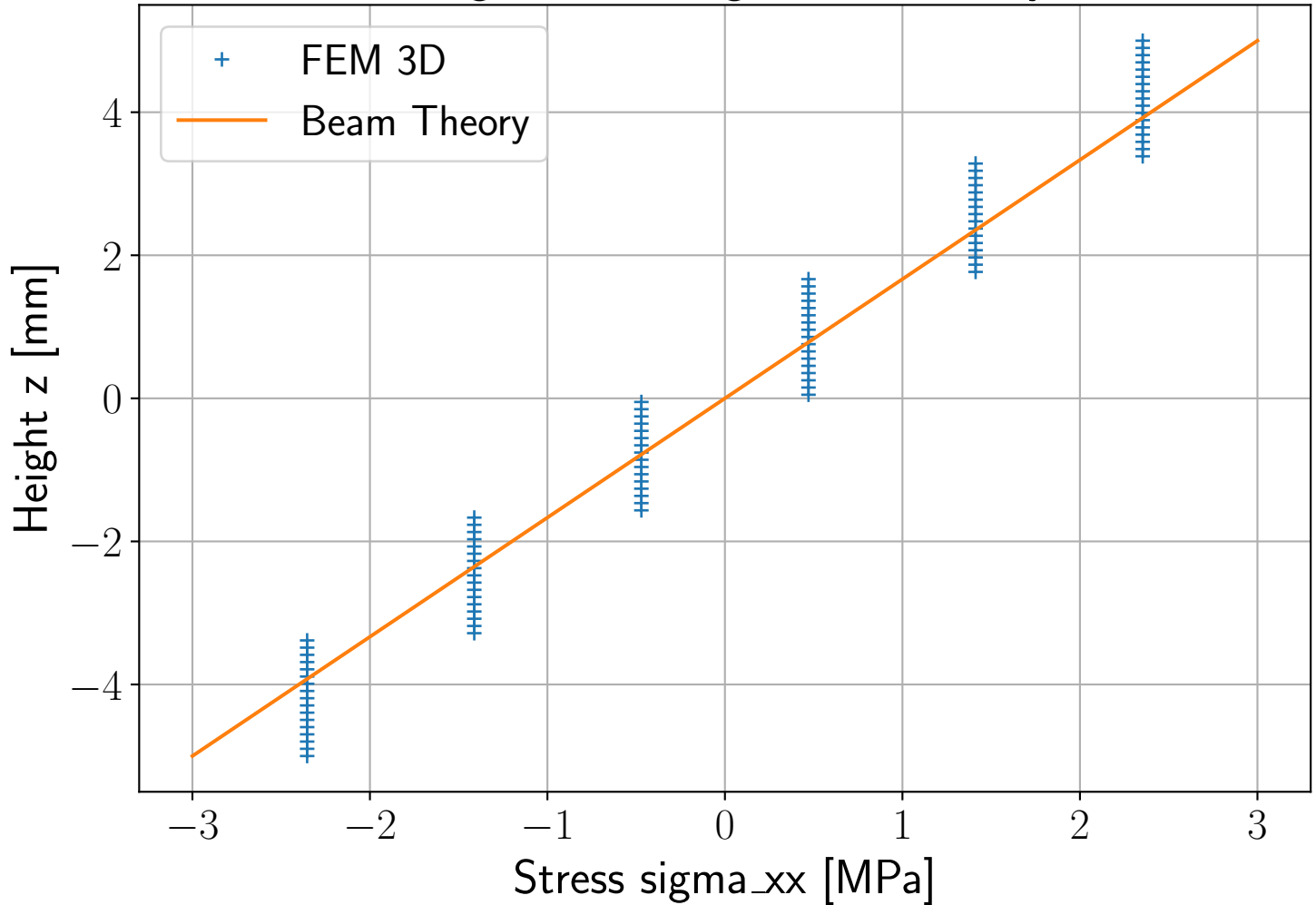
Stress \sigma_{xx} along z at x=500 , y=5.0
