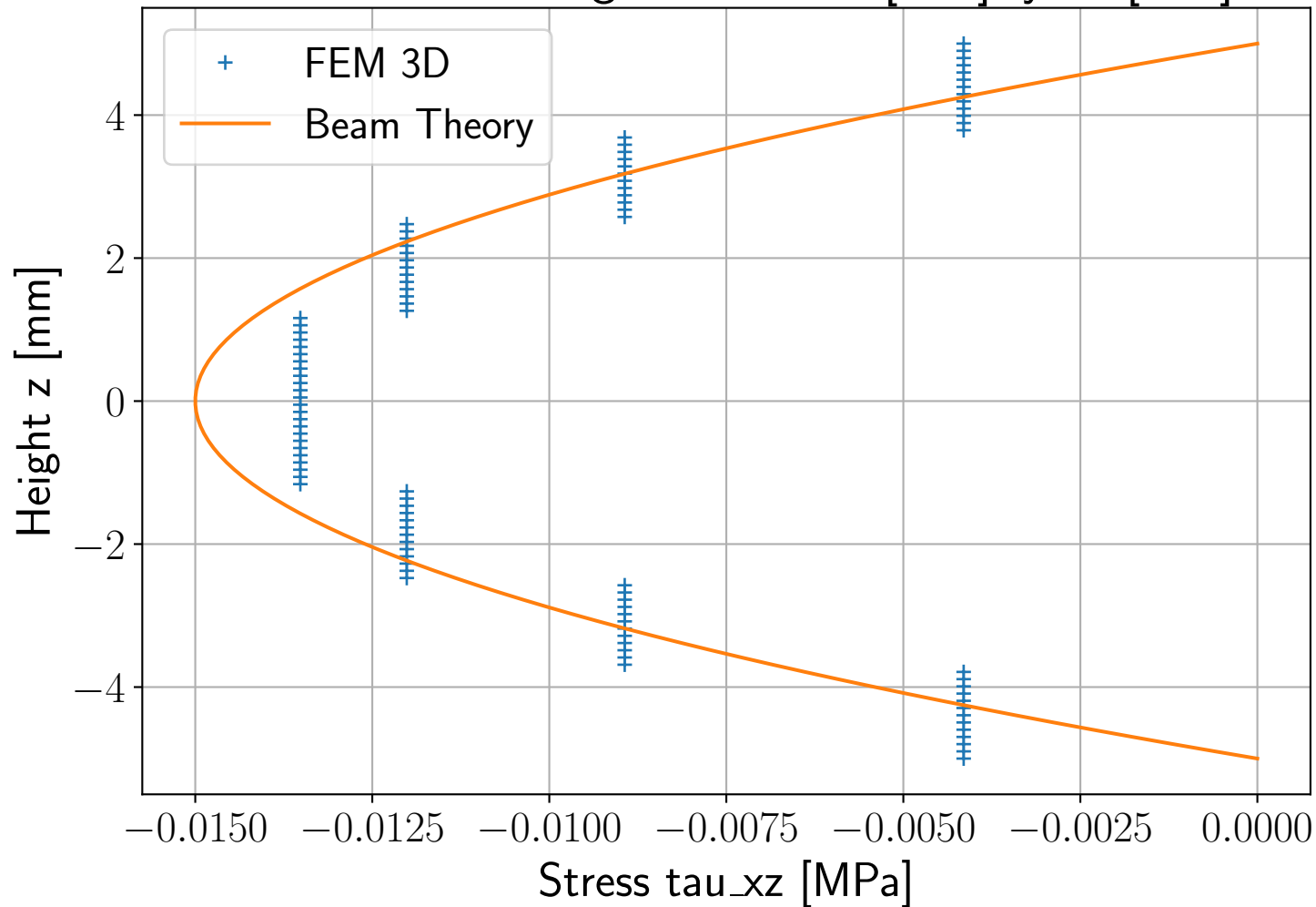
Stress \tau_{xz} along z at x=999 [mm], y=0 [mm]
