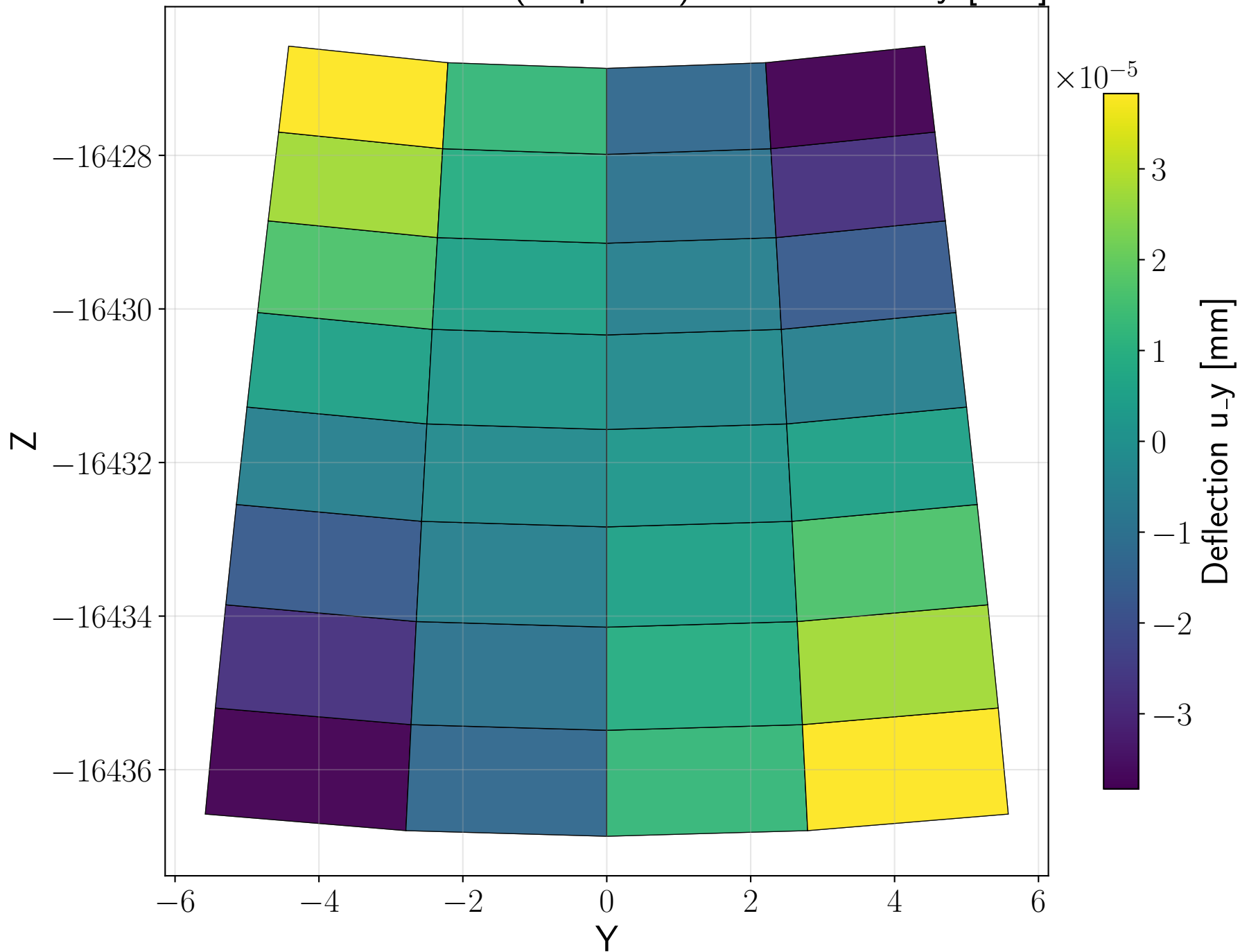
Slice at X = 500.000 (Displaced) - Deflection u_y [mm]
