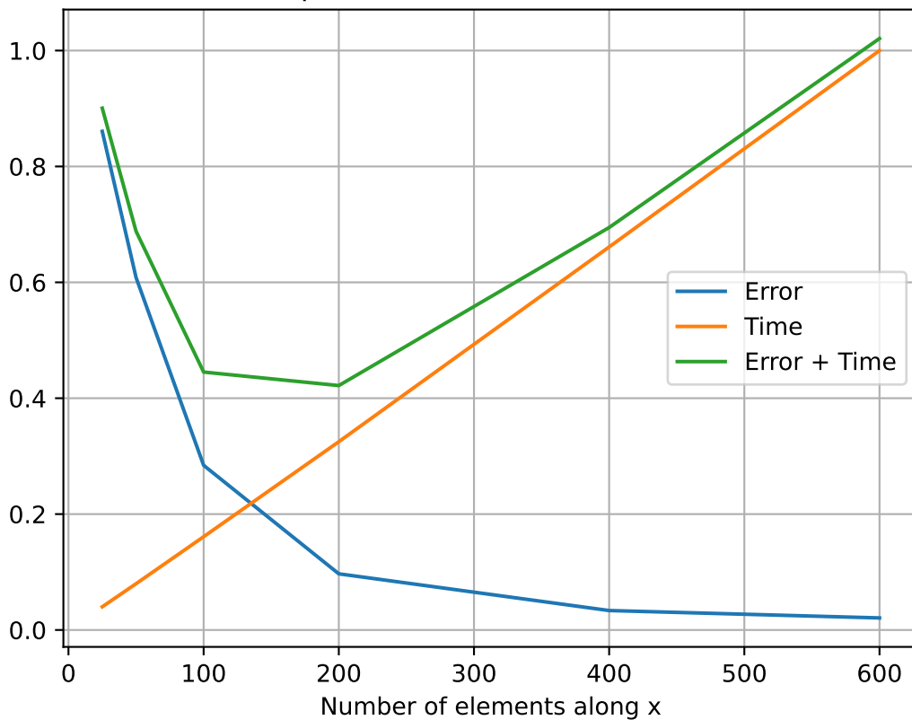
Error/Computational Time vs Mesh Refinement
