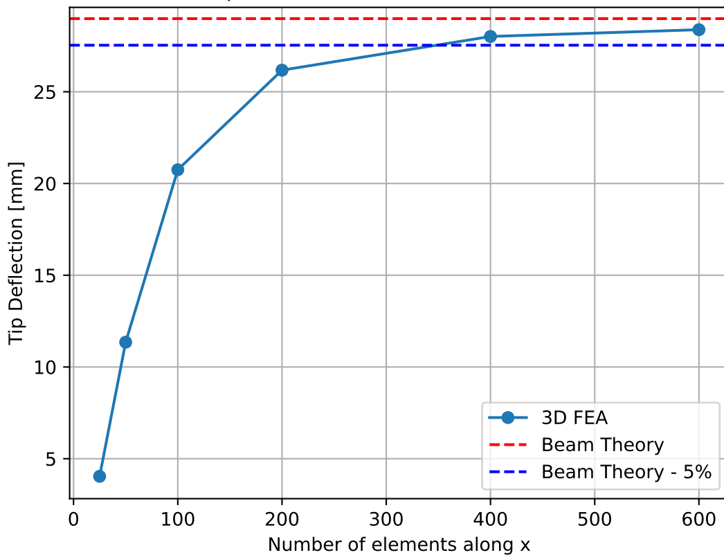
Tip Deflection vs Mesh Refinement
