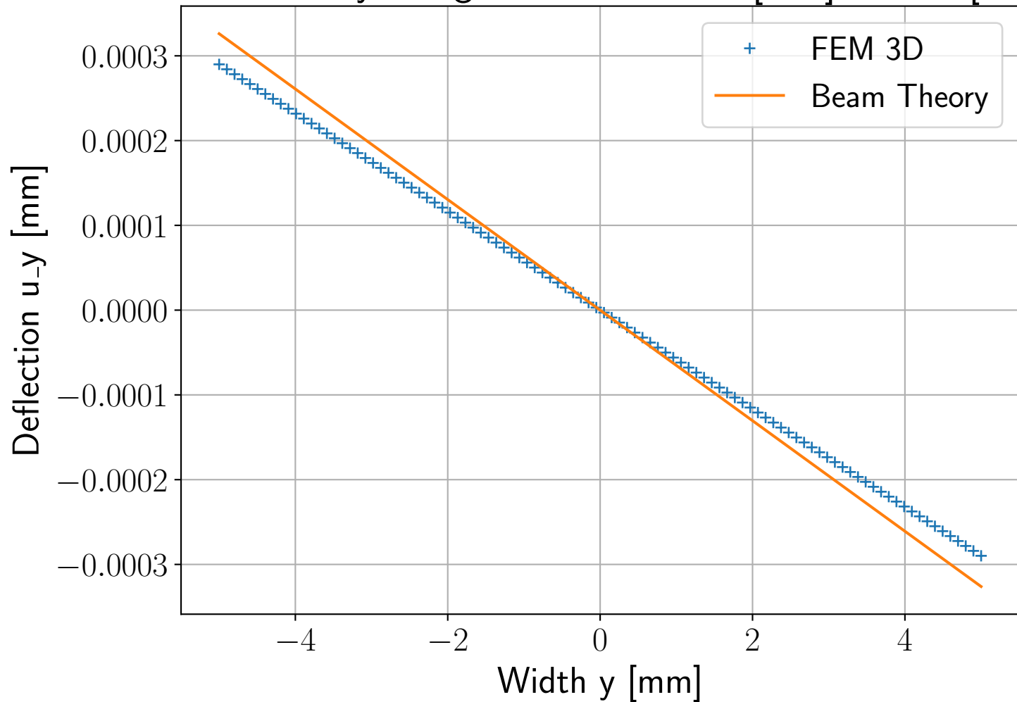
Deflection u_y along width at x=500 [mm], z=5.0 [mm]
