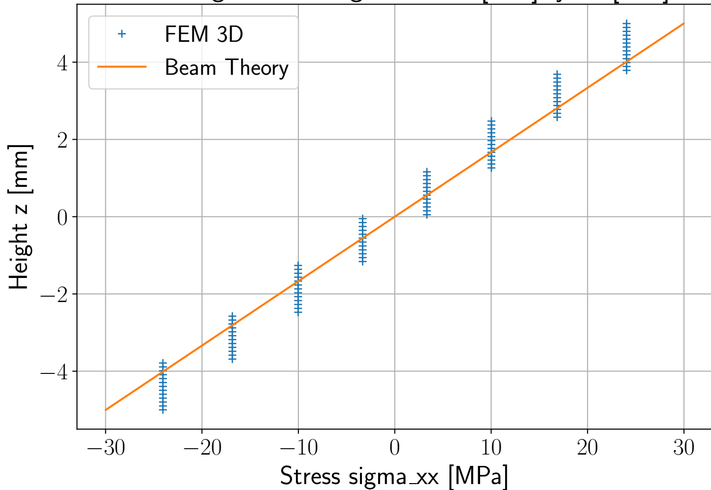
Stress \sigma_{xx} along z at x=1 [mm], y=0 [mm]
