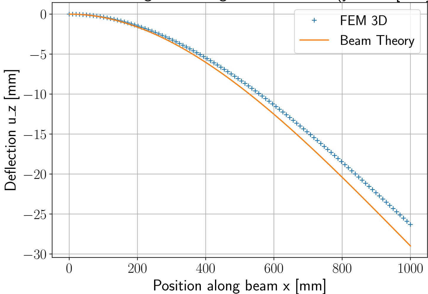
Deflection along beam length at centerline ( y=z=0 [mm])
