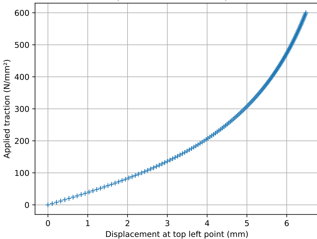
Load-Displacement Curve at Top Left Point
