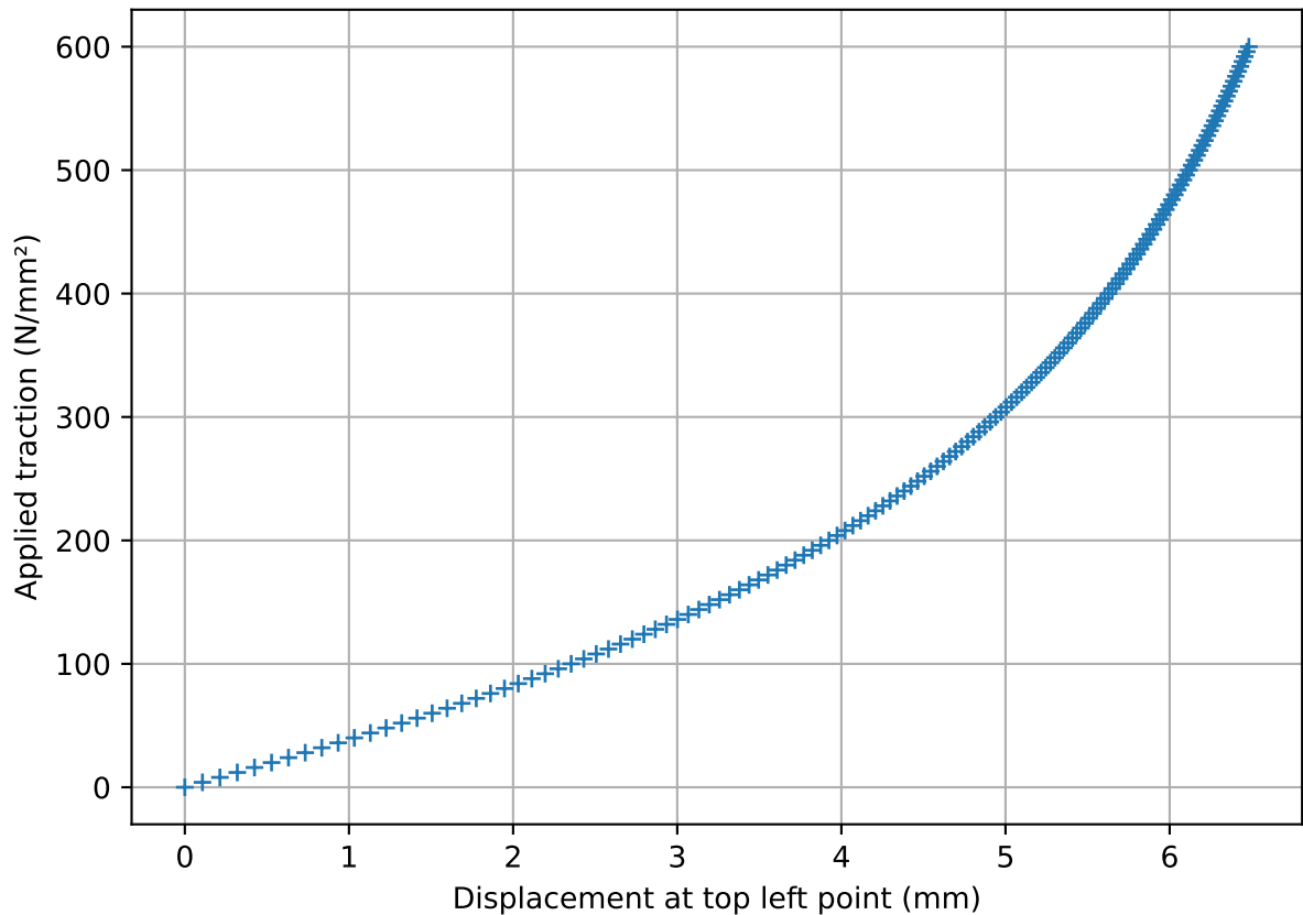
Load-Displacement Curve at Top Left Point
