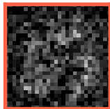
x_t (t=62)
