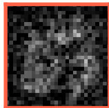
x_0 (final)
