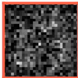
x_t (t=125)
