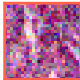
x_0 (final)
