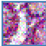
x_t (t=75)
