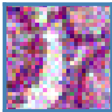
x_t (t=112)
