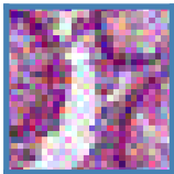
x_t (t=150)
