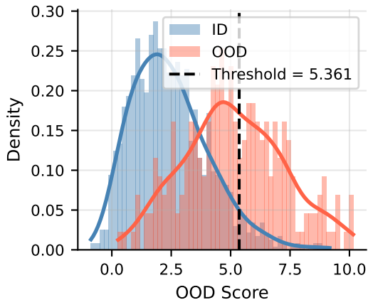
Score Distribution
