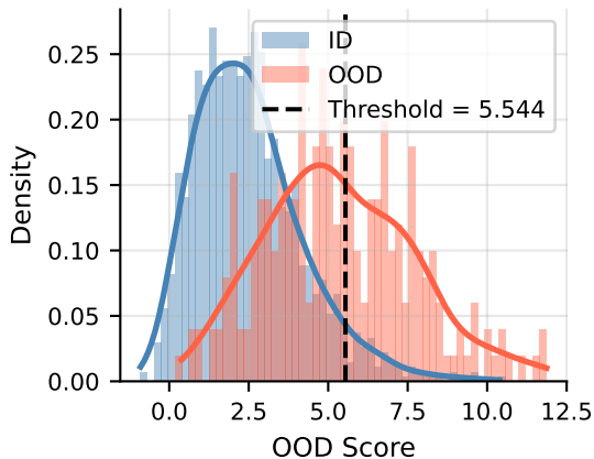
Score Distribution
