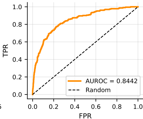
ROC Curve
