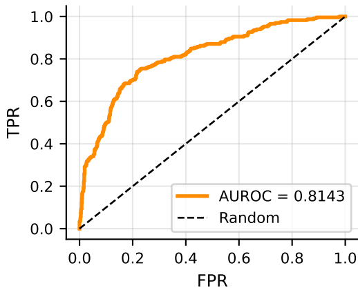
ROC Curve
