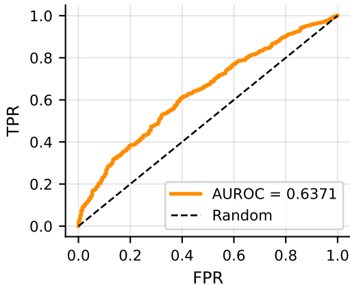
ROC Curve
