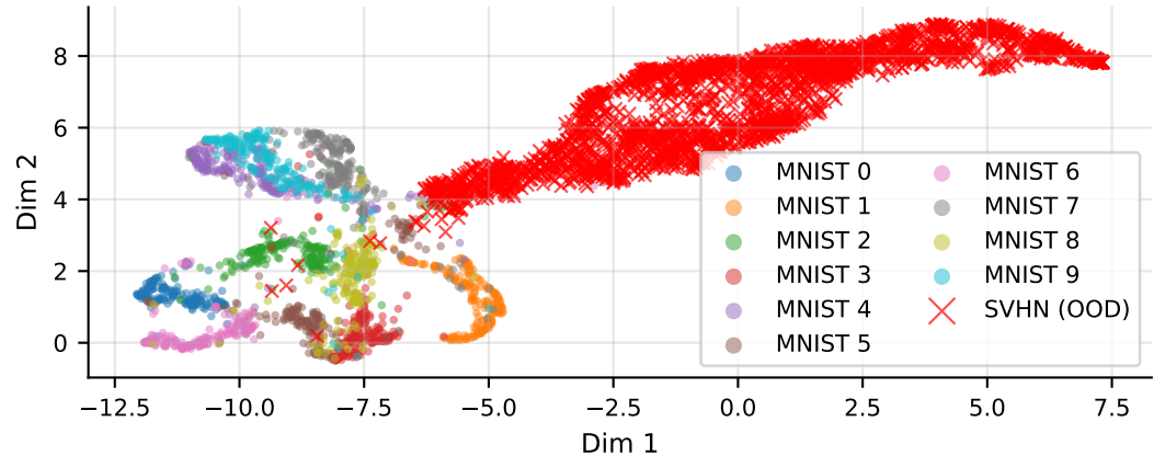
UMAP (2D)
