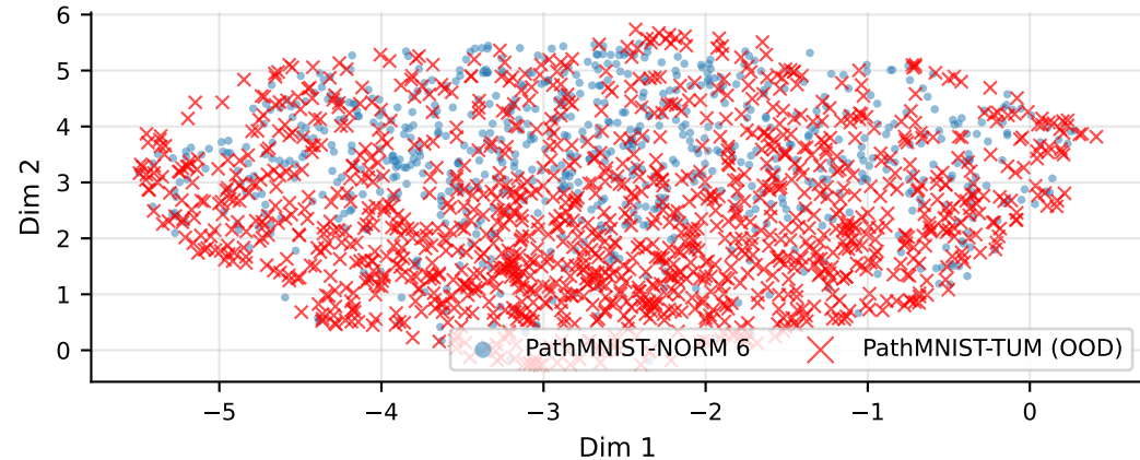
UMAP (2D)
