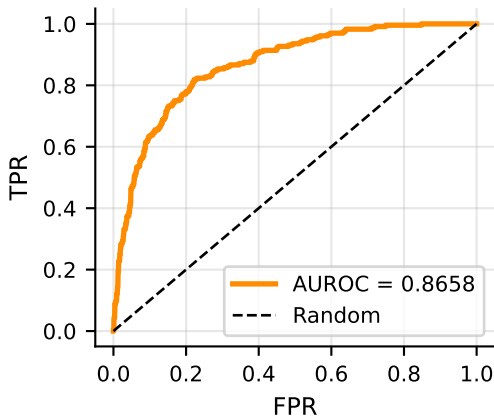
ROC Curve
