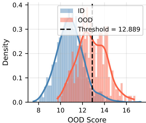
Score Distribution
