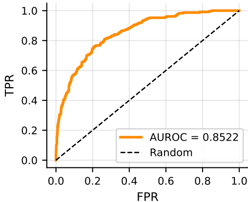
ROC Curve
