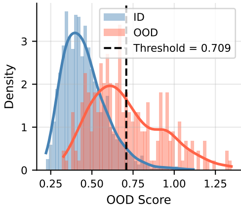
Score Distribution
