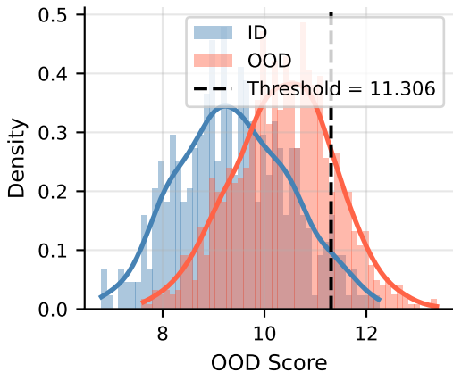
Score Distribution
