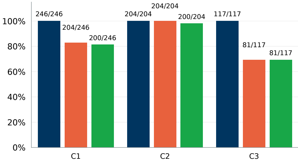
Accuracy on applicable checks
