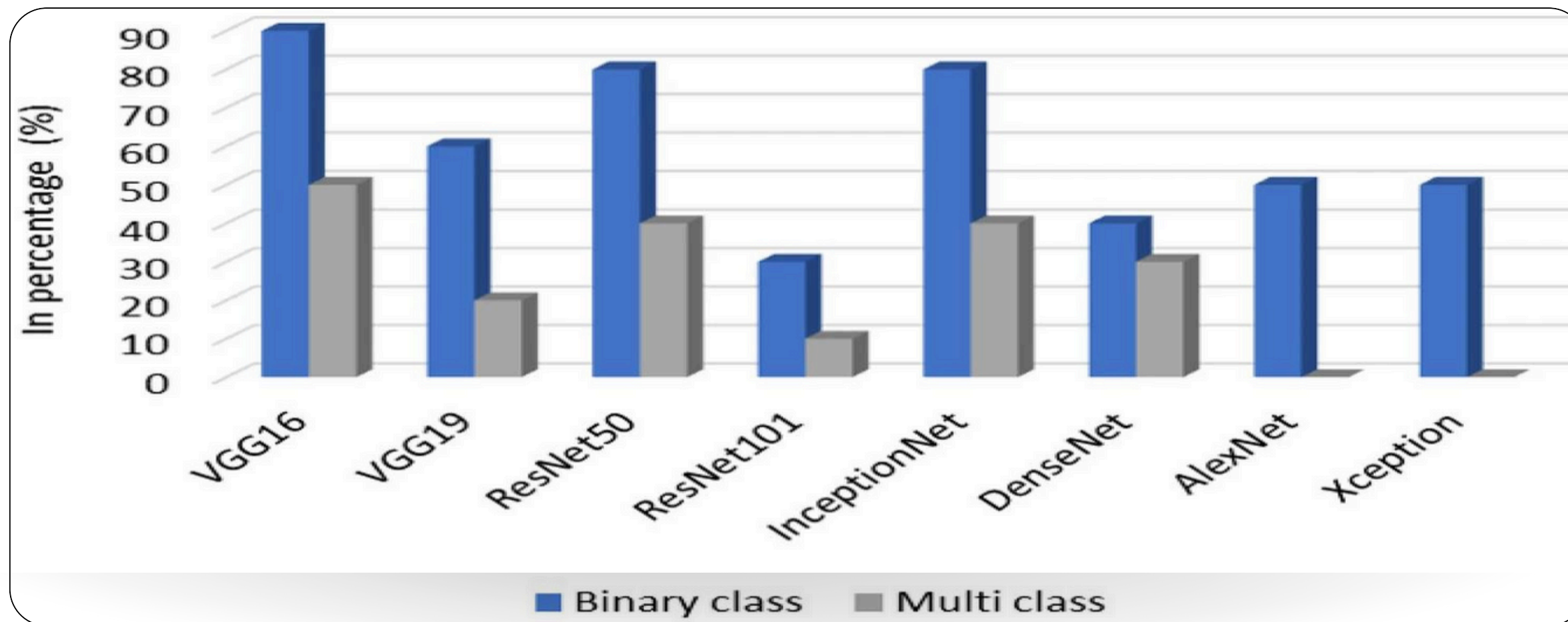
Figure 2: Various CNN Architectures for Binary and Multi-Class Classification, Specifically for Breast Cancer Histopathological Images
