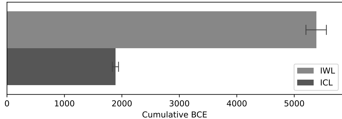
Omniglot
