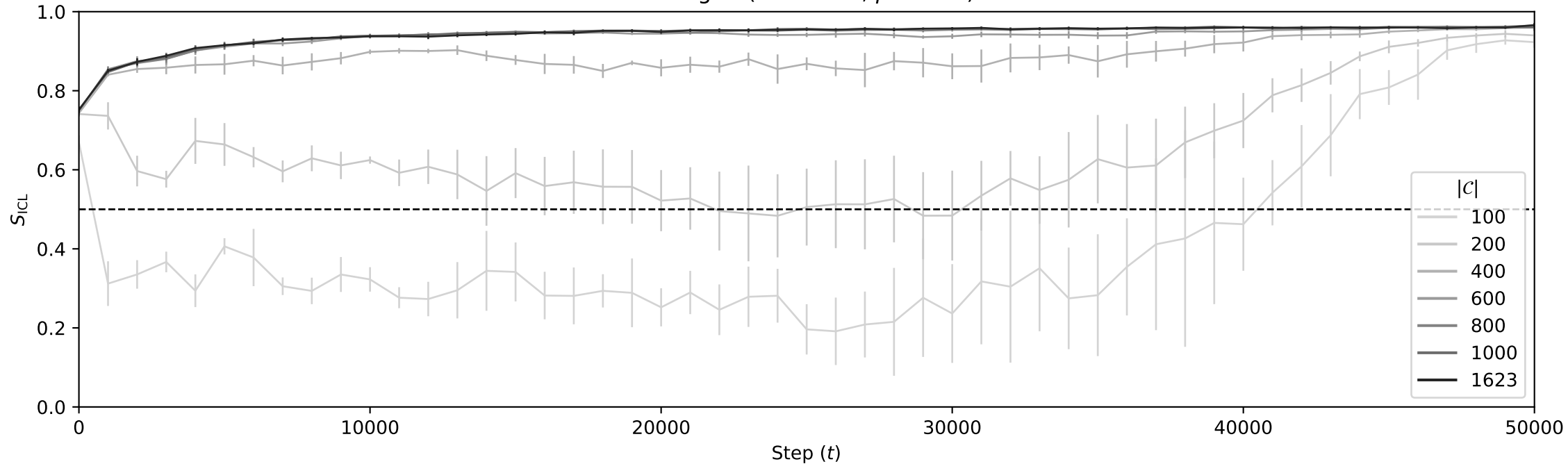
Omniglot ( \alpha = 0.999, \rho = 0.95 )
