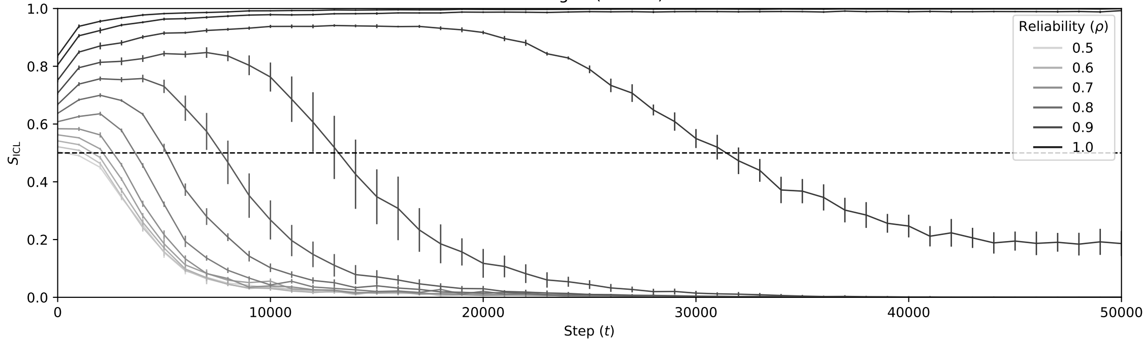
Omniglot ( \alpha = 1.0 )
