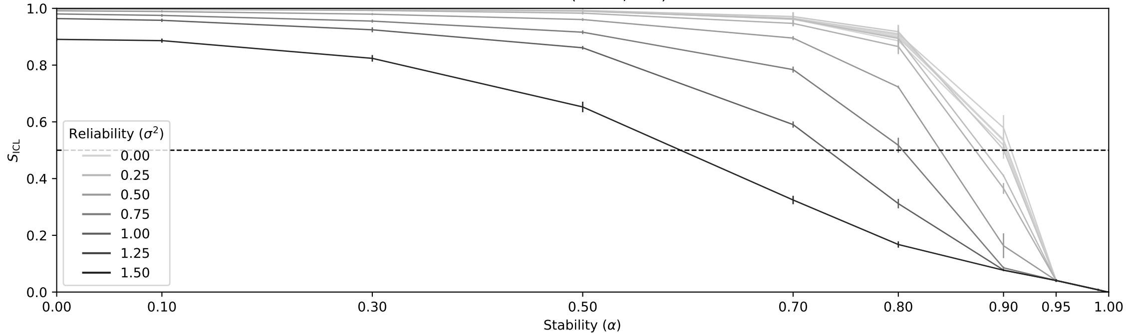
Sinusoid ( t = 50,000 )
