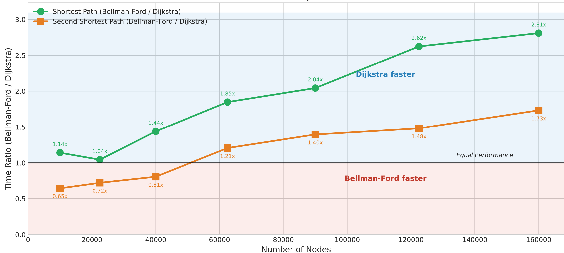
Performance Ratio: Queue-Optimized Bellman-Ford vs Dijkstra on Grid Graphs (Ratio > 1 means Dijkstra is faster)
