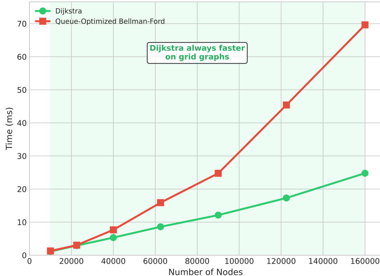
Shortest Path (Grid Graph)
