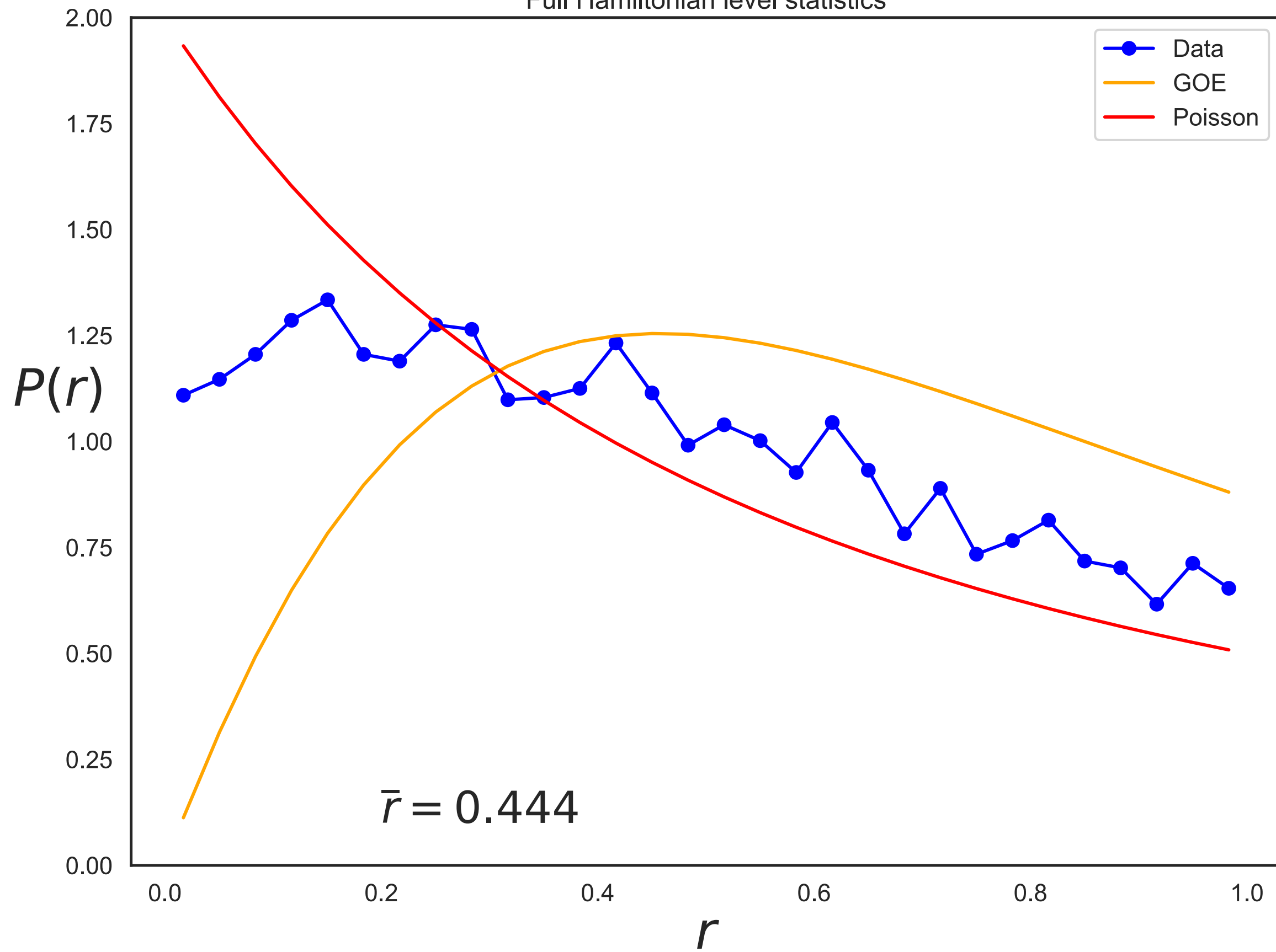
Full Hamiltonian level statistics
