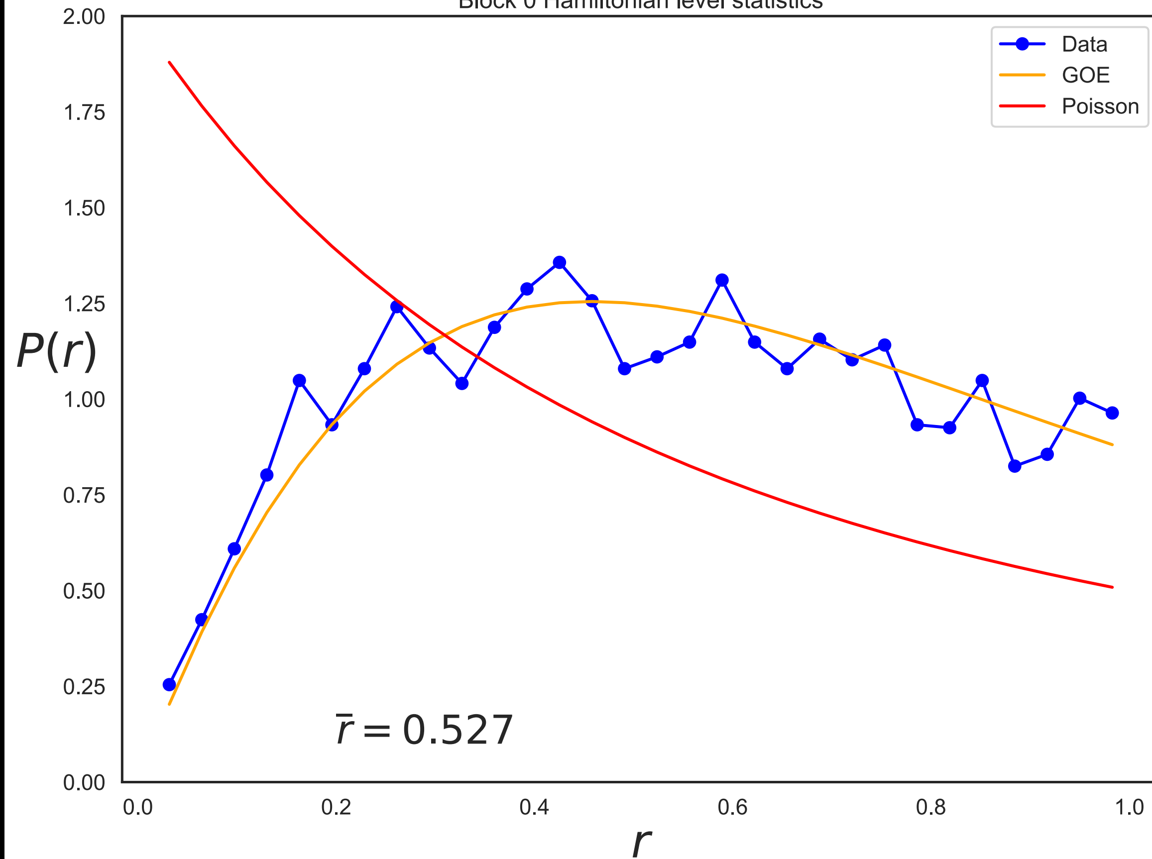
Block 0 Hamiltonian level statistics
