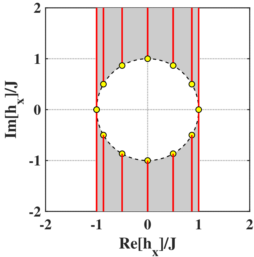
(b) Odd Parity Sector (PBC)
