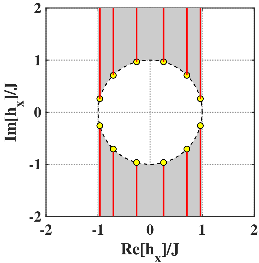
(a) Even Parity Sector (APBC)
