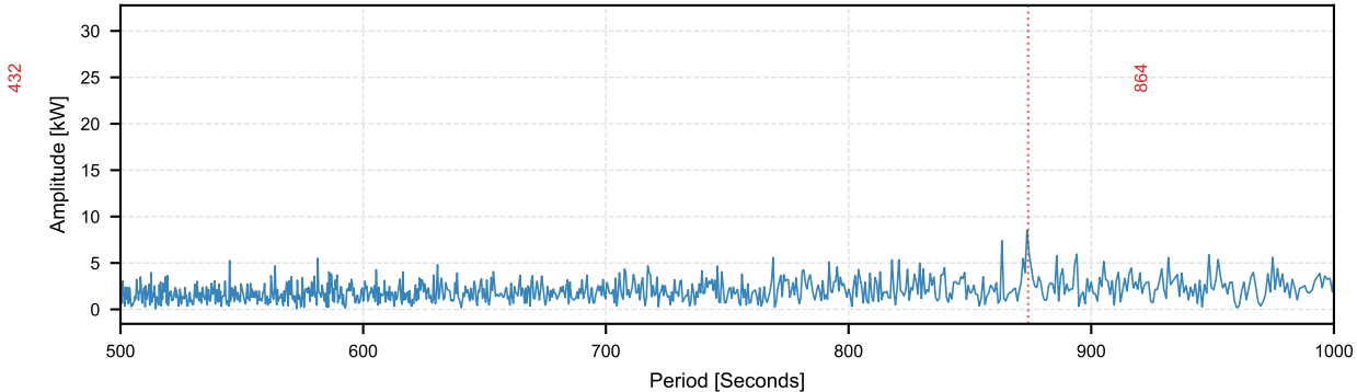
Sub 1-Hour Spectral Energy of Fleet Power Demand
