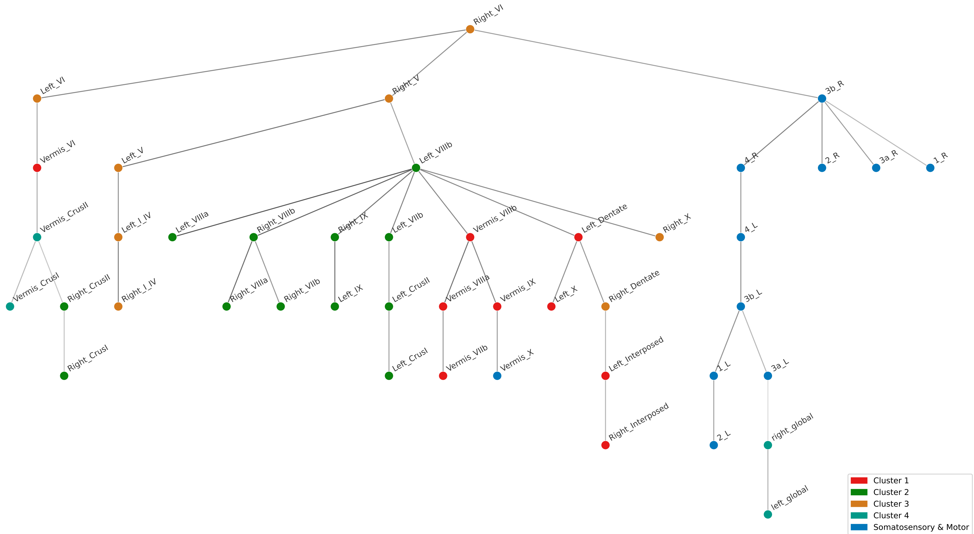
Chow-Liu Tree (Cluster Coloring) – MSC04
