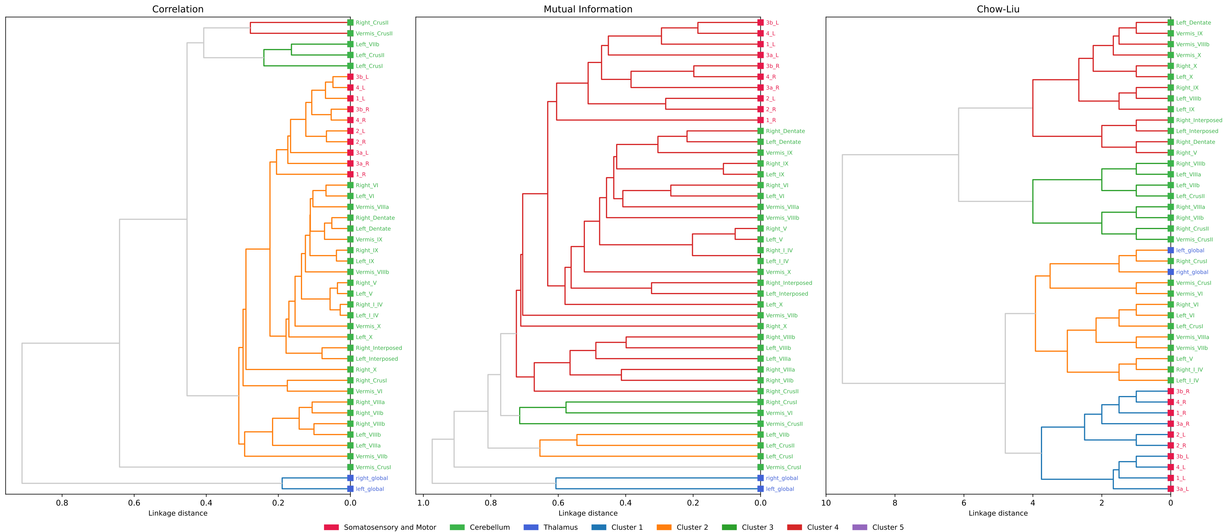
Labeled Dendrograms (Shared Leaf Order = Correlation) — MSC09 (k = 5) Branch color = each method's k-cluster | Right strips: cluster color (inner) and known network (outer)
