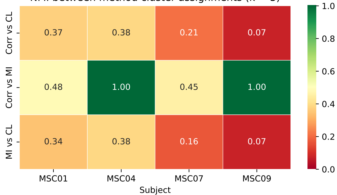
NMI between method cluster assignments (k = 3)
