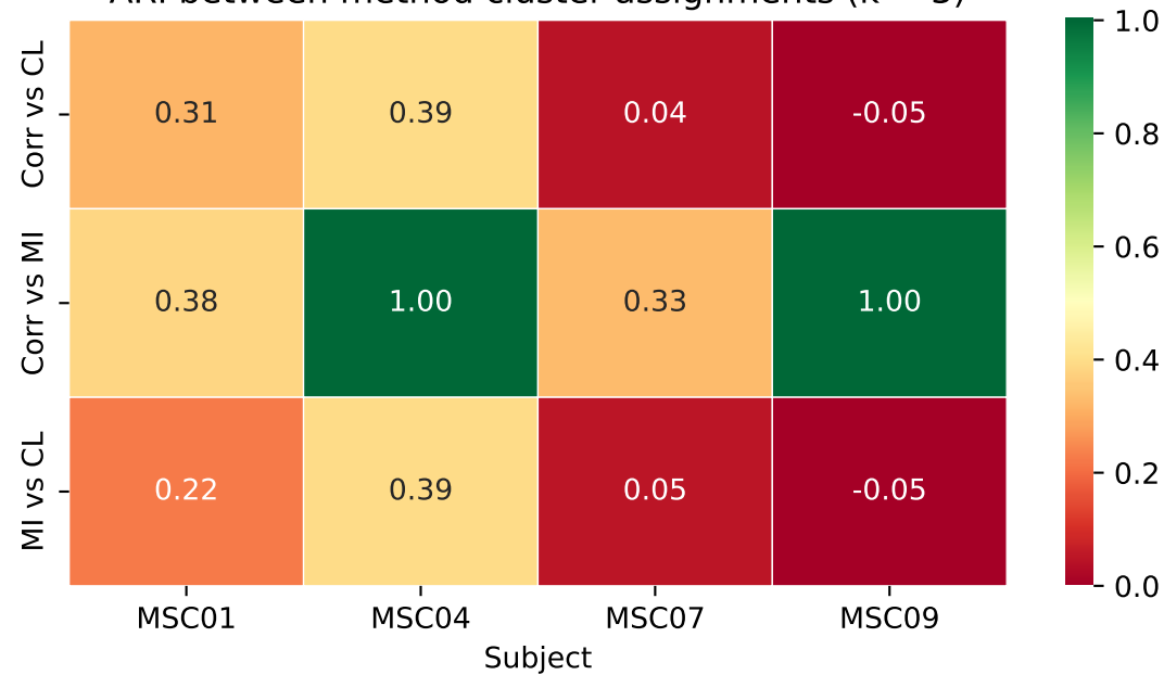
ARI between method cluster assignments (k = 3)
