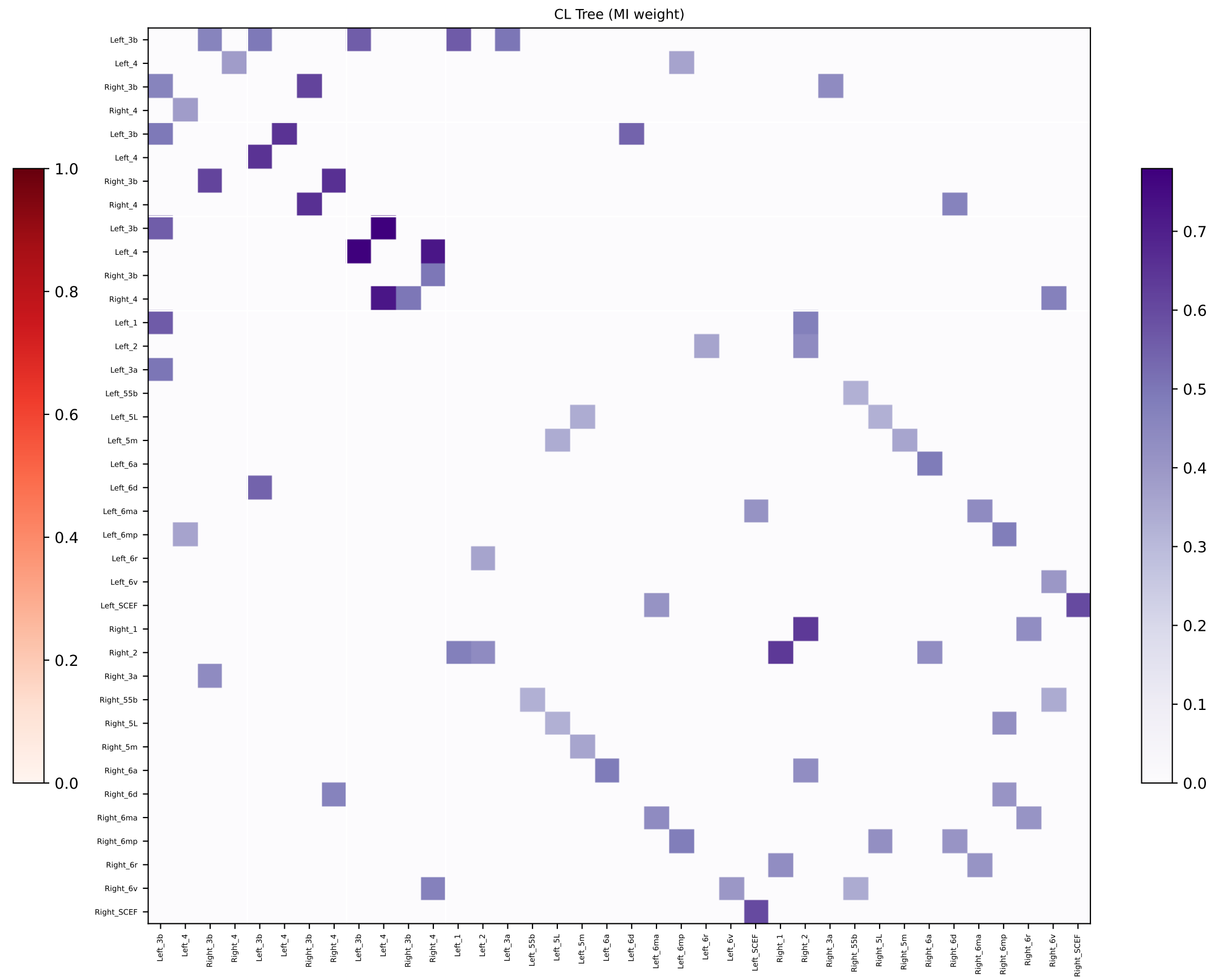
MSC01 — Localizer Motor ROIs: FC vs CL Adjacency
