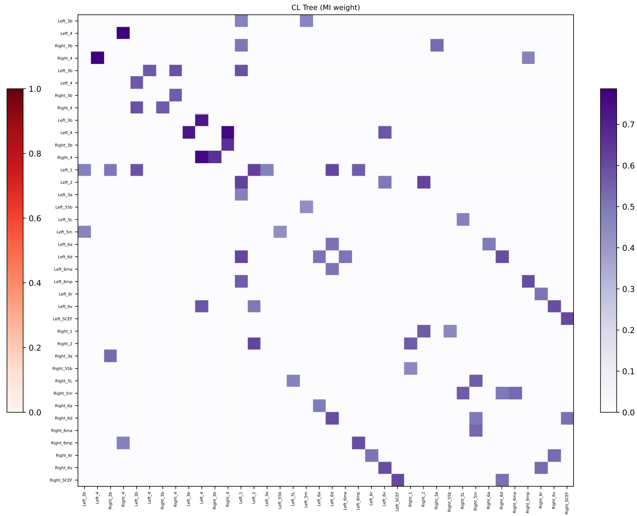
MSC04 — Localizer Motor ROIs: FC vs CL Adjacency
