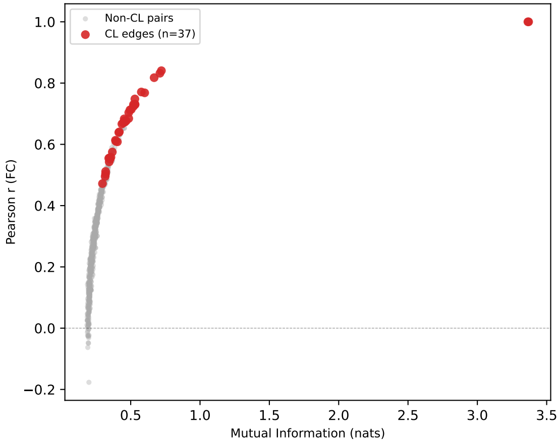
MSC05 — FC vs MI for Localizer Motor ROIs
