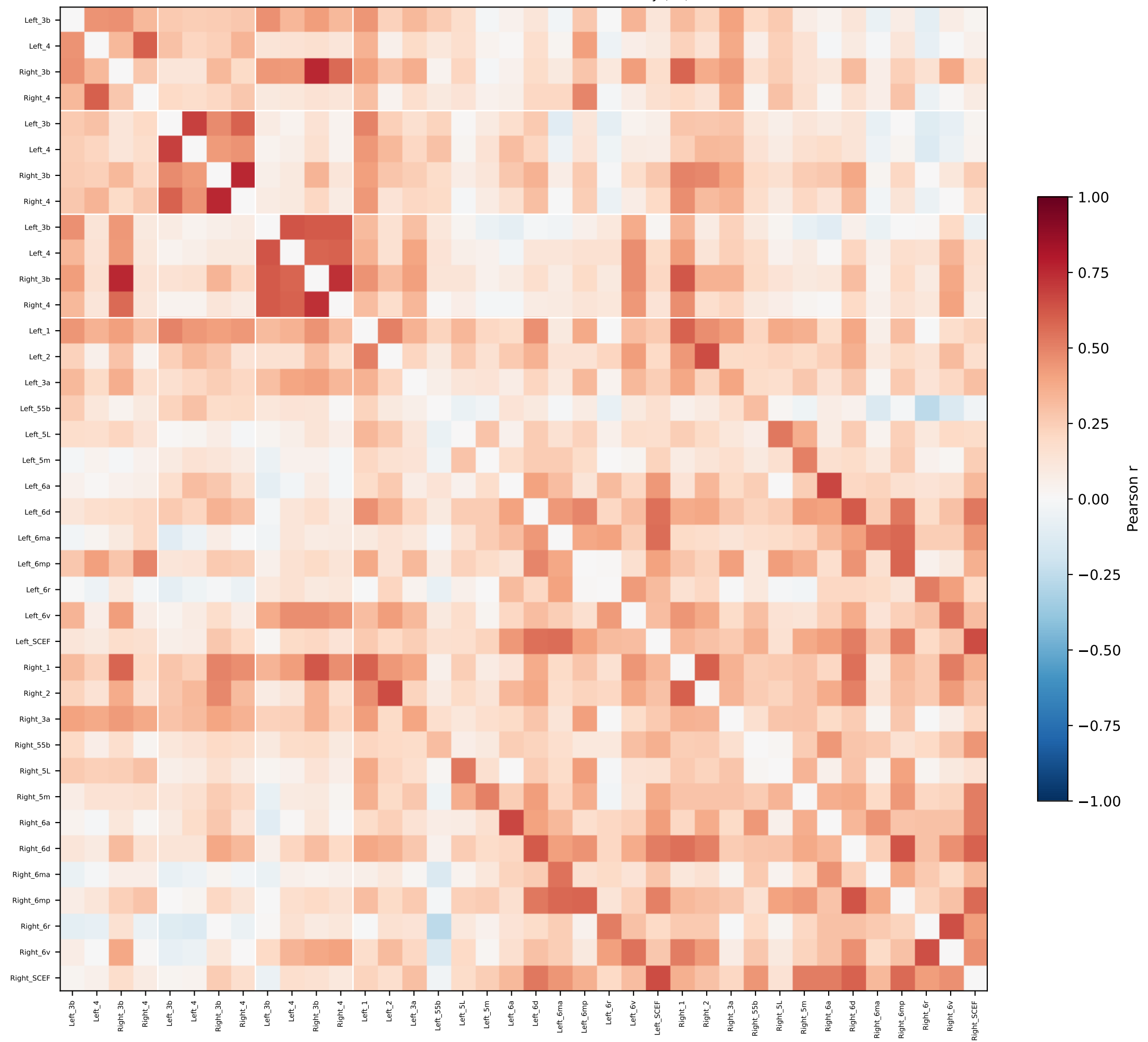
MSC06 — Localizer ROI Functional Connectivity (FC)
