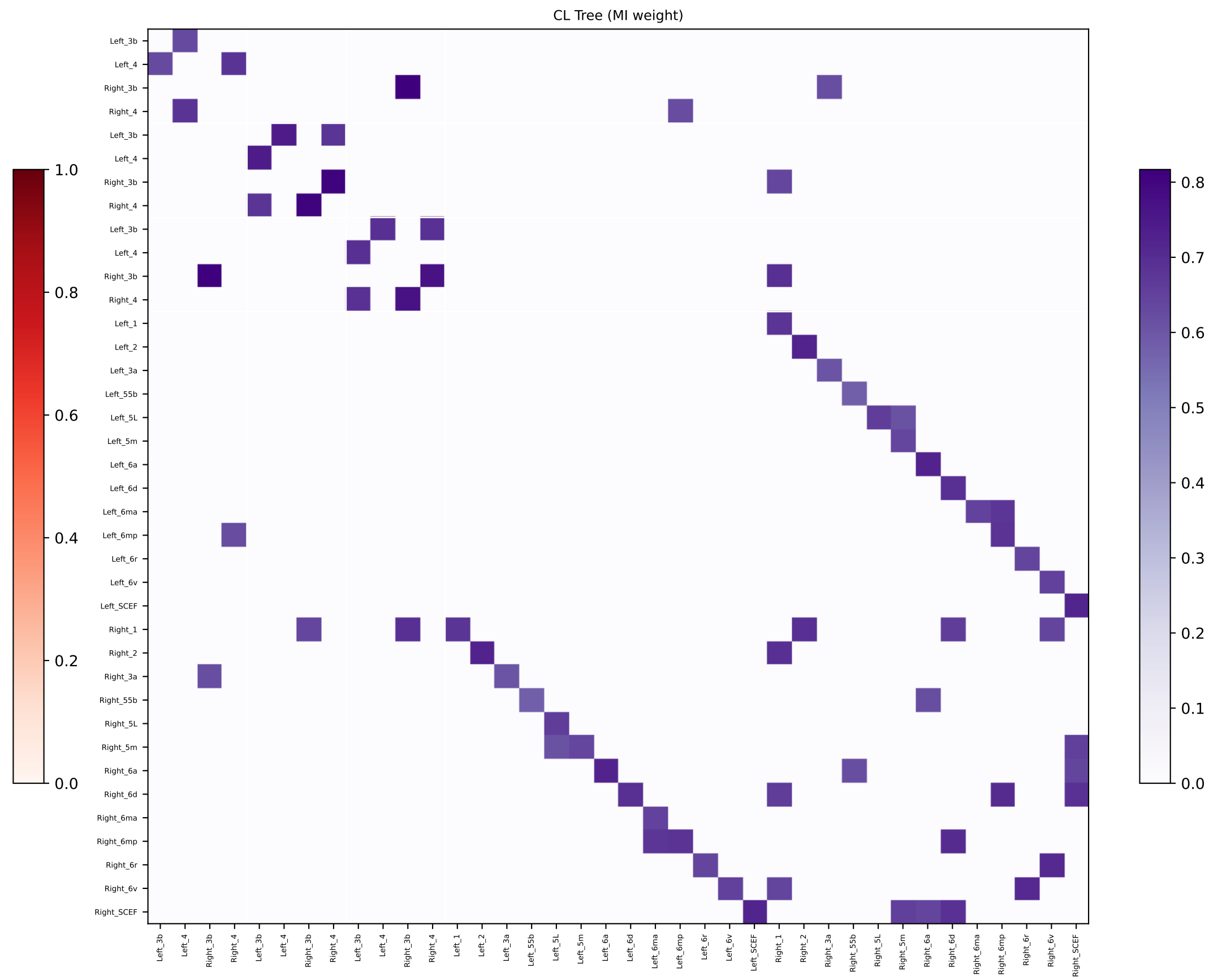
MSC06 — Localizer Motor ROIs: FC vs CL Adjacency
