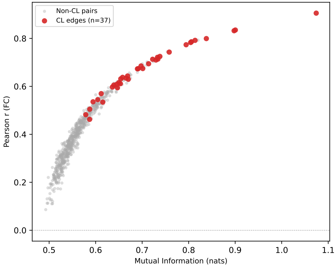
MSC08 — FC vs MI for Localizer Motor ROIs
