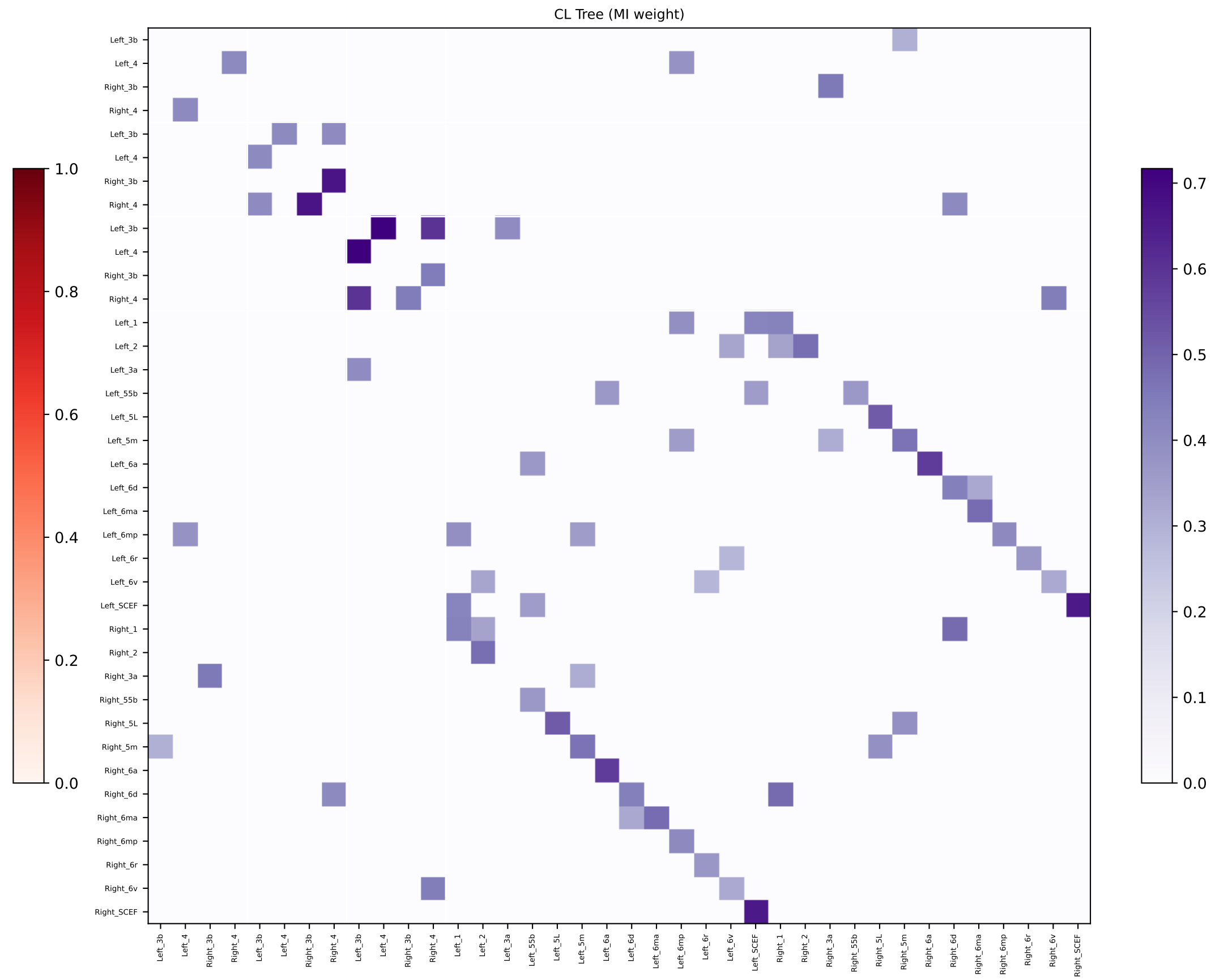
MSC09 — Localizer Motor ROIs: FC vs CL Adjacency
