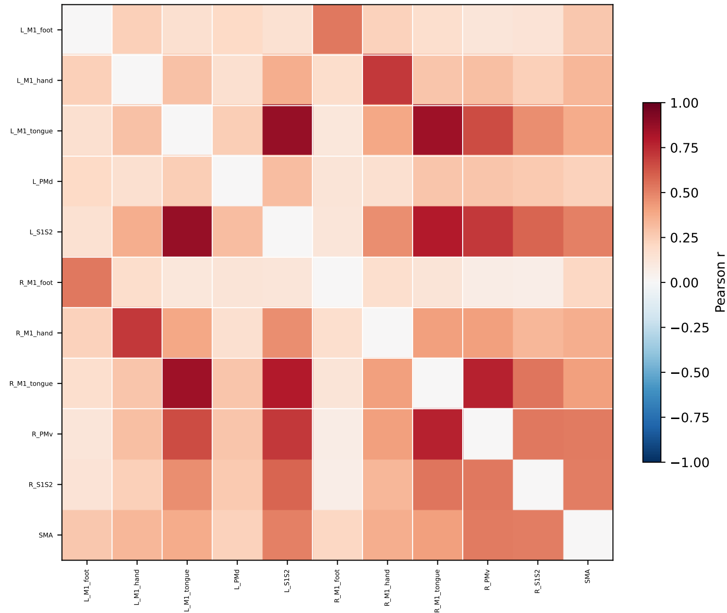
MSC02_all_sessions — GCSS Motor FC
