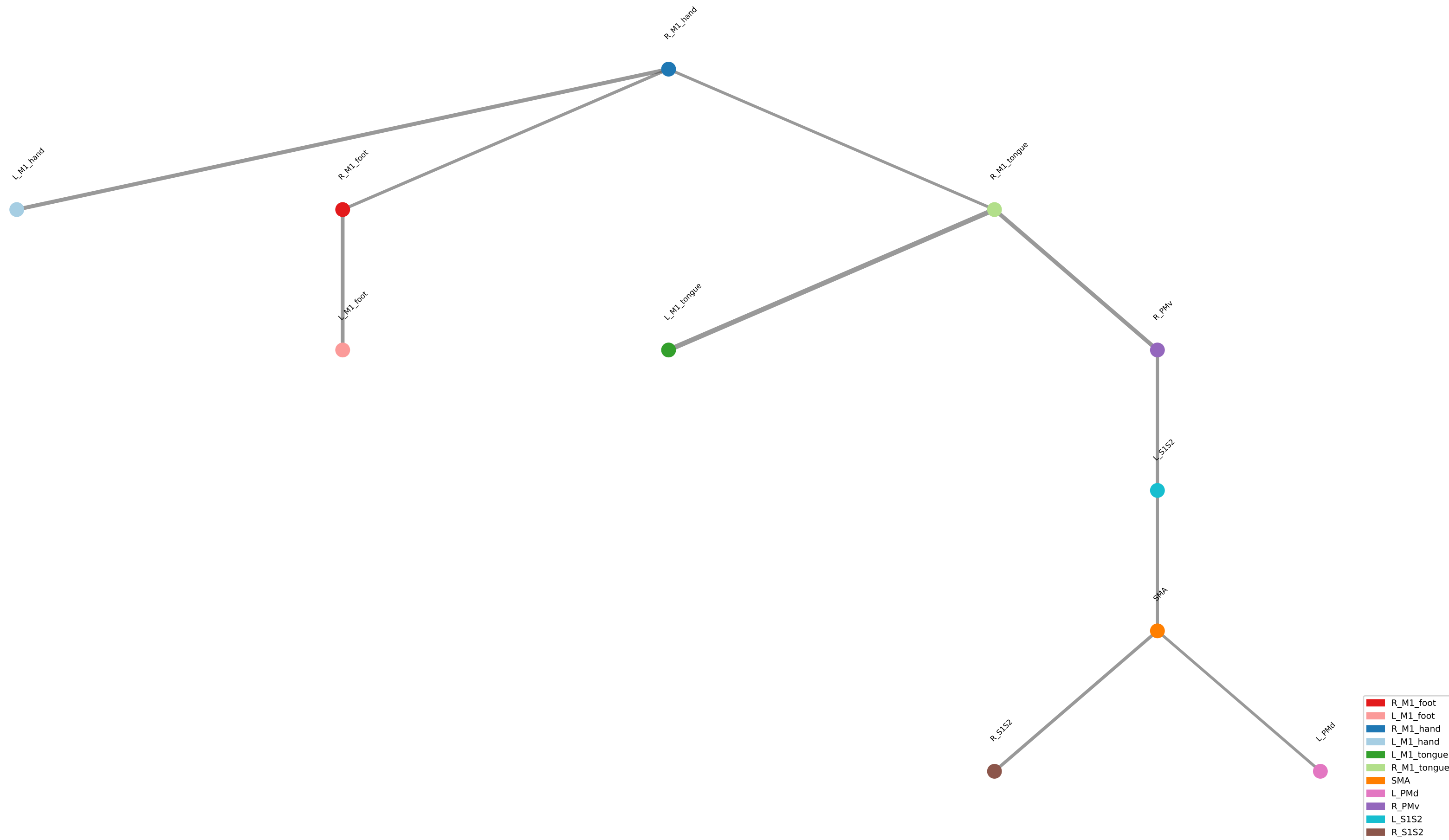
MSC05_all_sessions — GCSS Motor CL Tree
