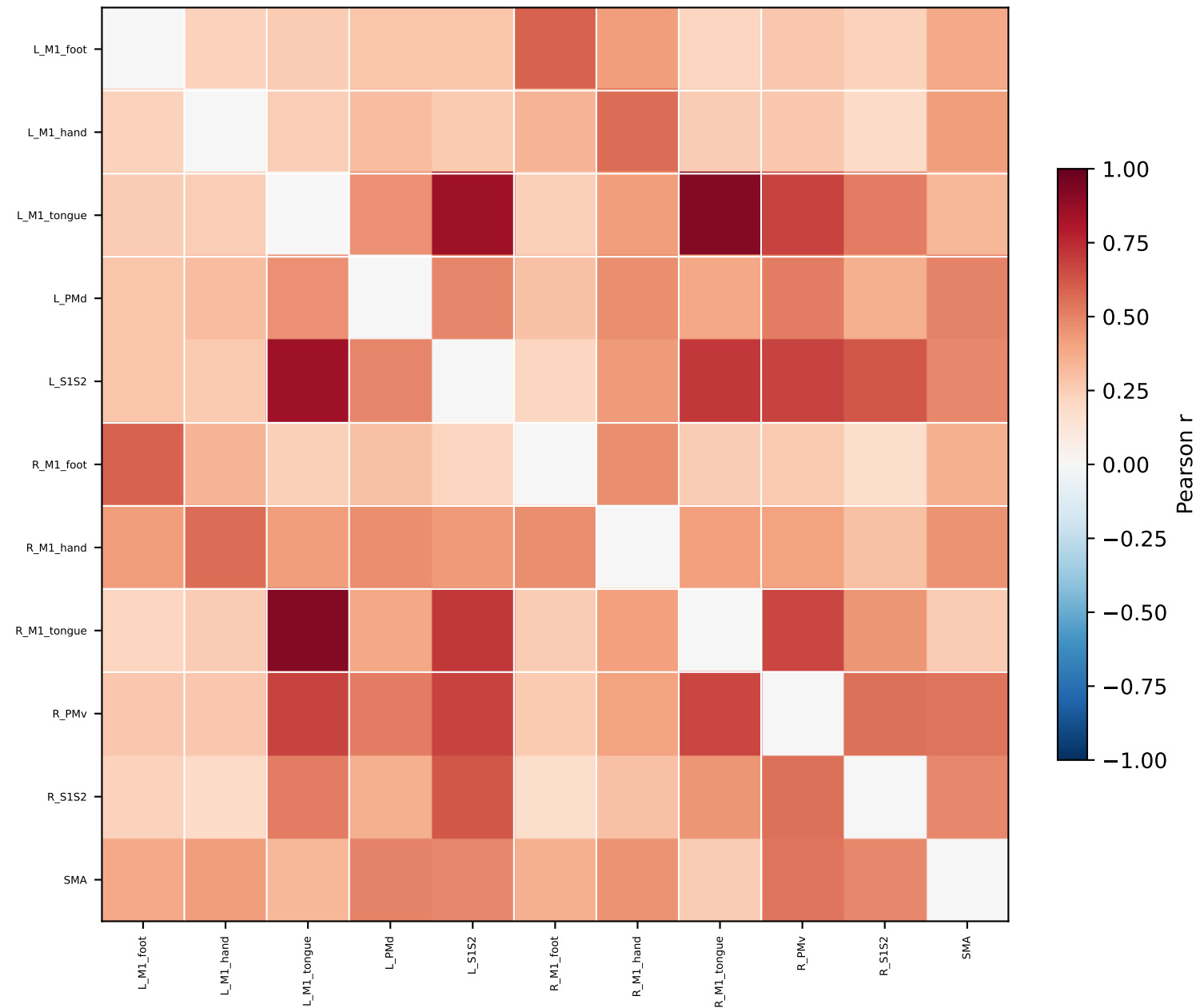
MSC10_all_sessions — GCSS Motor FC
