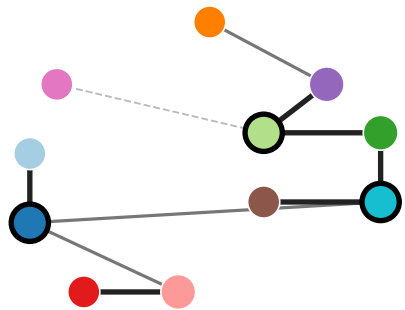
MSC07 ( \bar{M}\bar{I}=0.51 )
