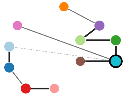
MSC08 ( \bar{M}\bar{I}=0.64 )
