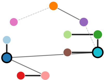
MSC06 ( \bar{M}\bar{I}=0.57 )
