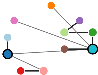
MSC09 ( \bar{M}\bar{I}=0.28 )
