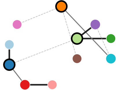
MSC10 ( \bar{M}\bar{I}=0.52 )
