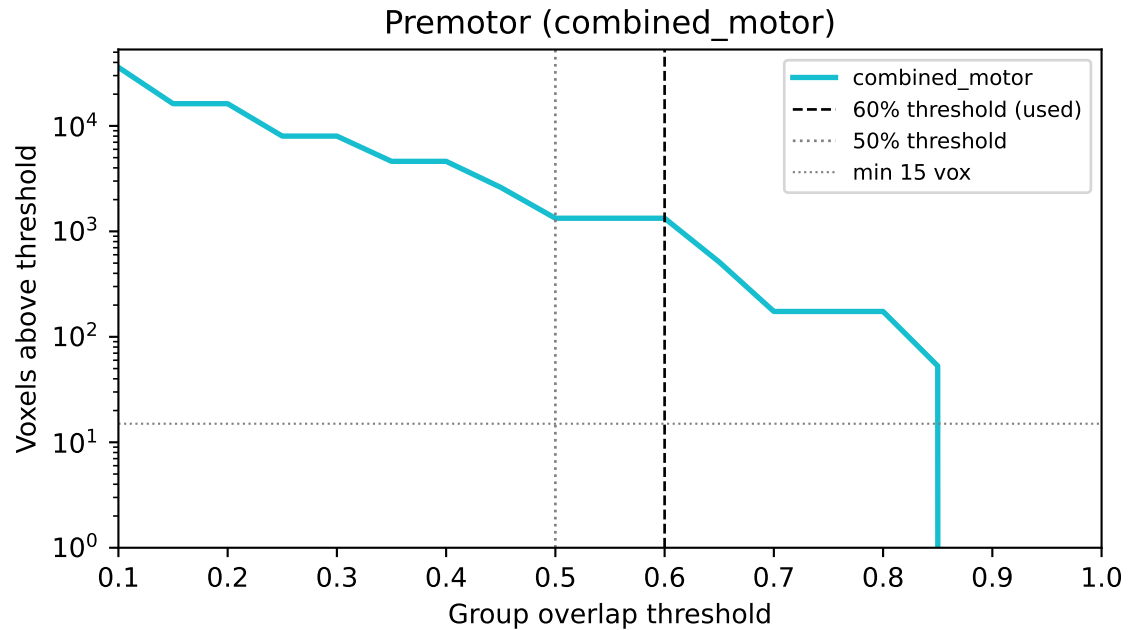
GCSS Group Probability Maps — Voxel Count vs. Threshold Dashed = 60% group-overlap cutoff used for clustering
