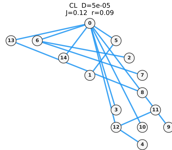
Recovered networks per individual (linear coupling, heterogeneous intrinsics) Row 1: Chow-Liu tree | Row 2: FC density tree (top N-1 edges)
