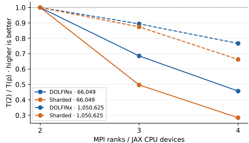
Communication scaling relative to 2 ranks
