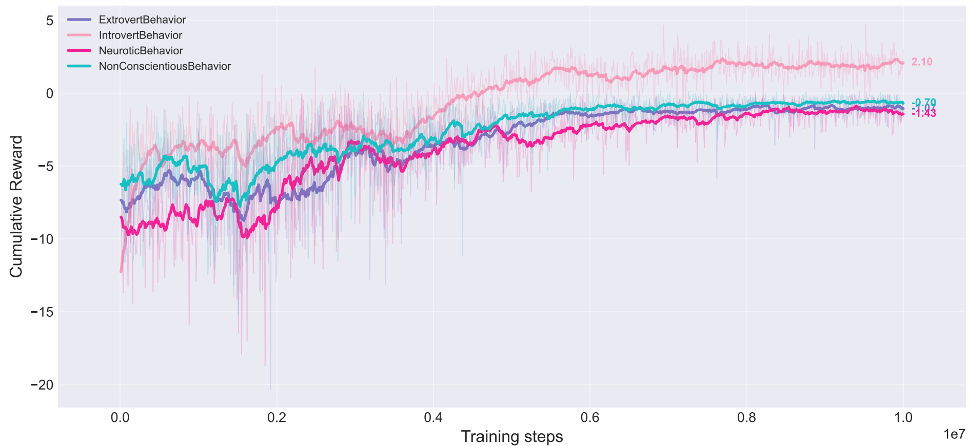
Cumulative Reward
